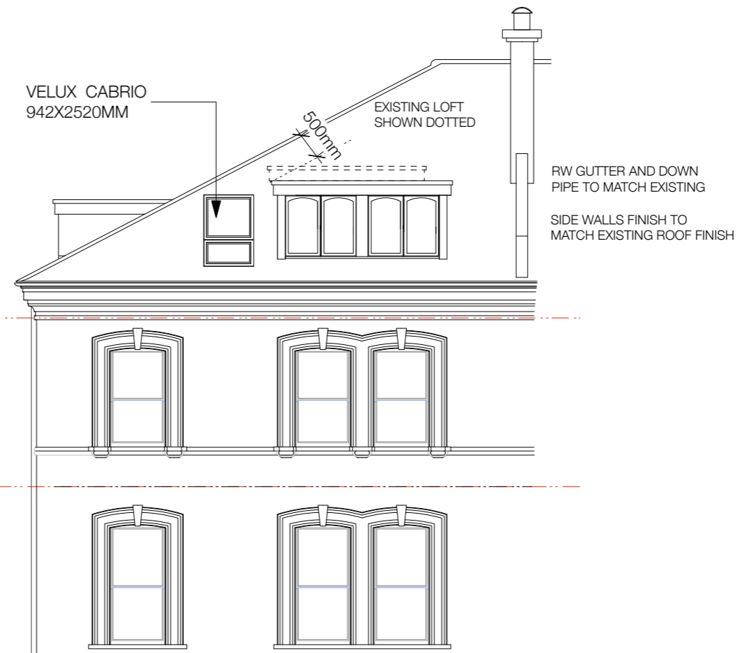
REAR ELEVATION
