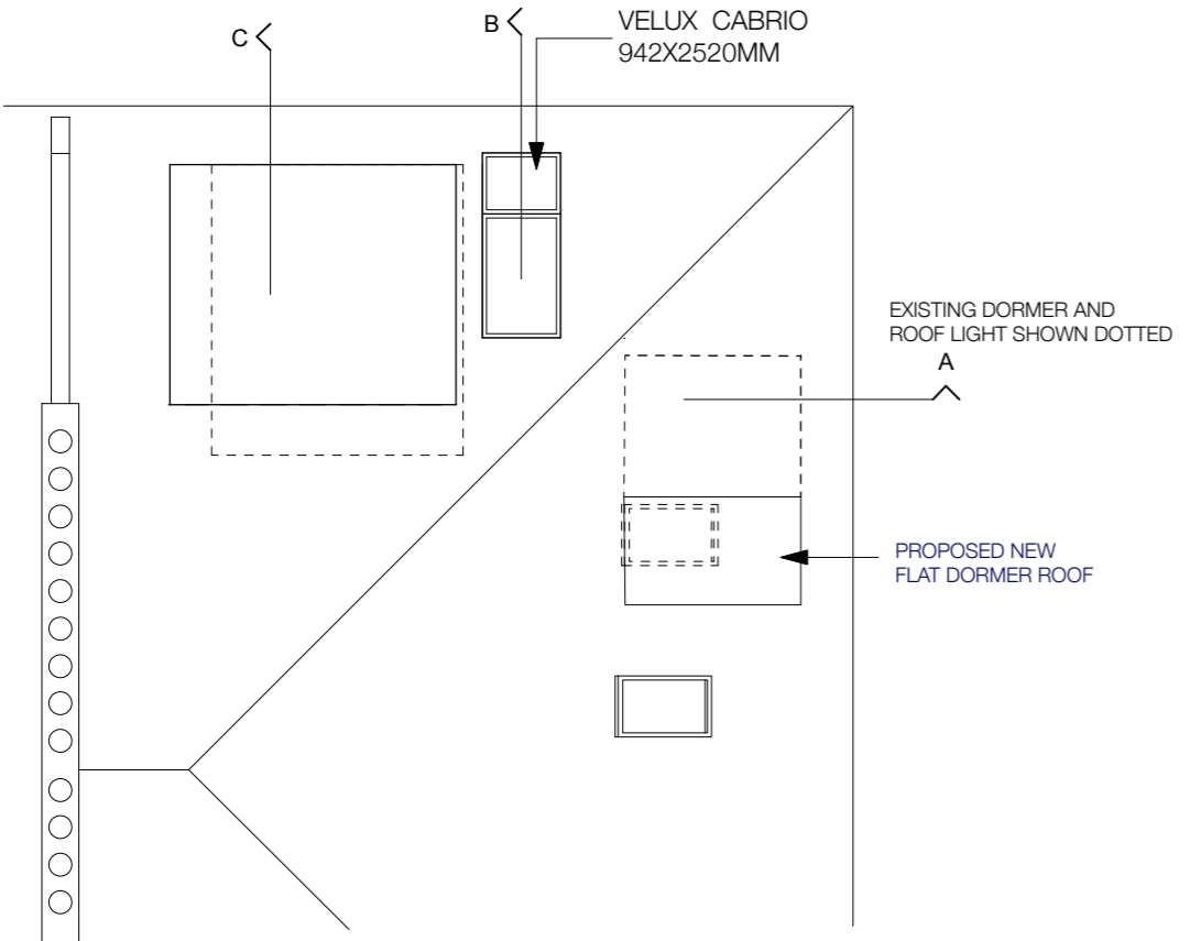
ROOF PLAN
