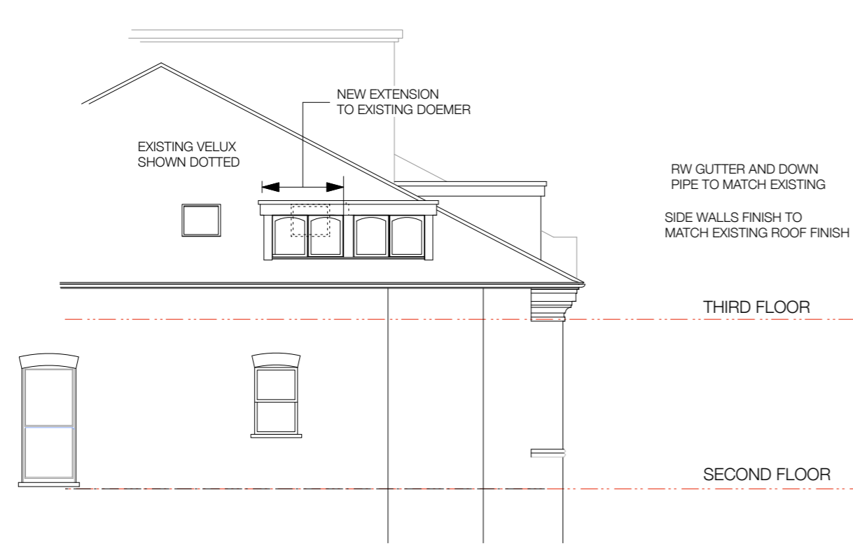
SIDE ELEVATION
