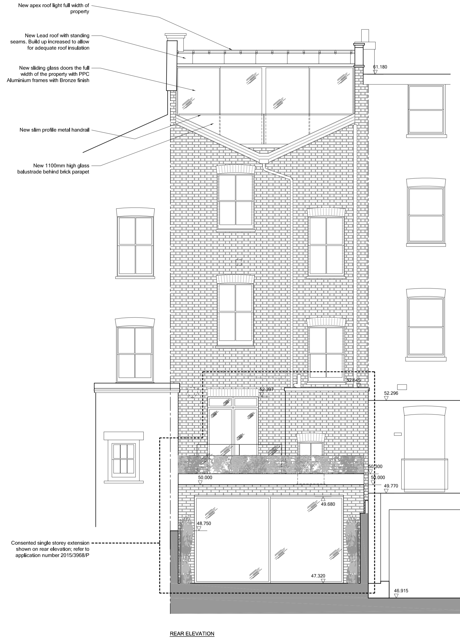
REAR ELEVATION
