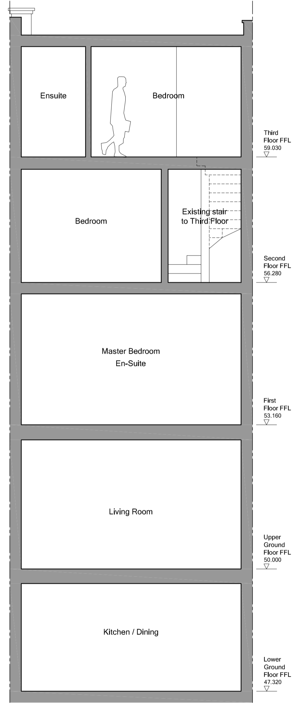
SECTION C-C
