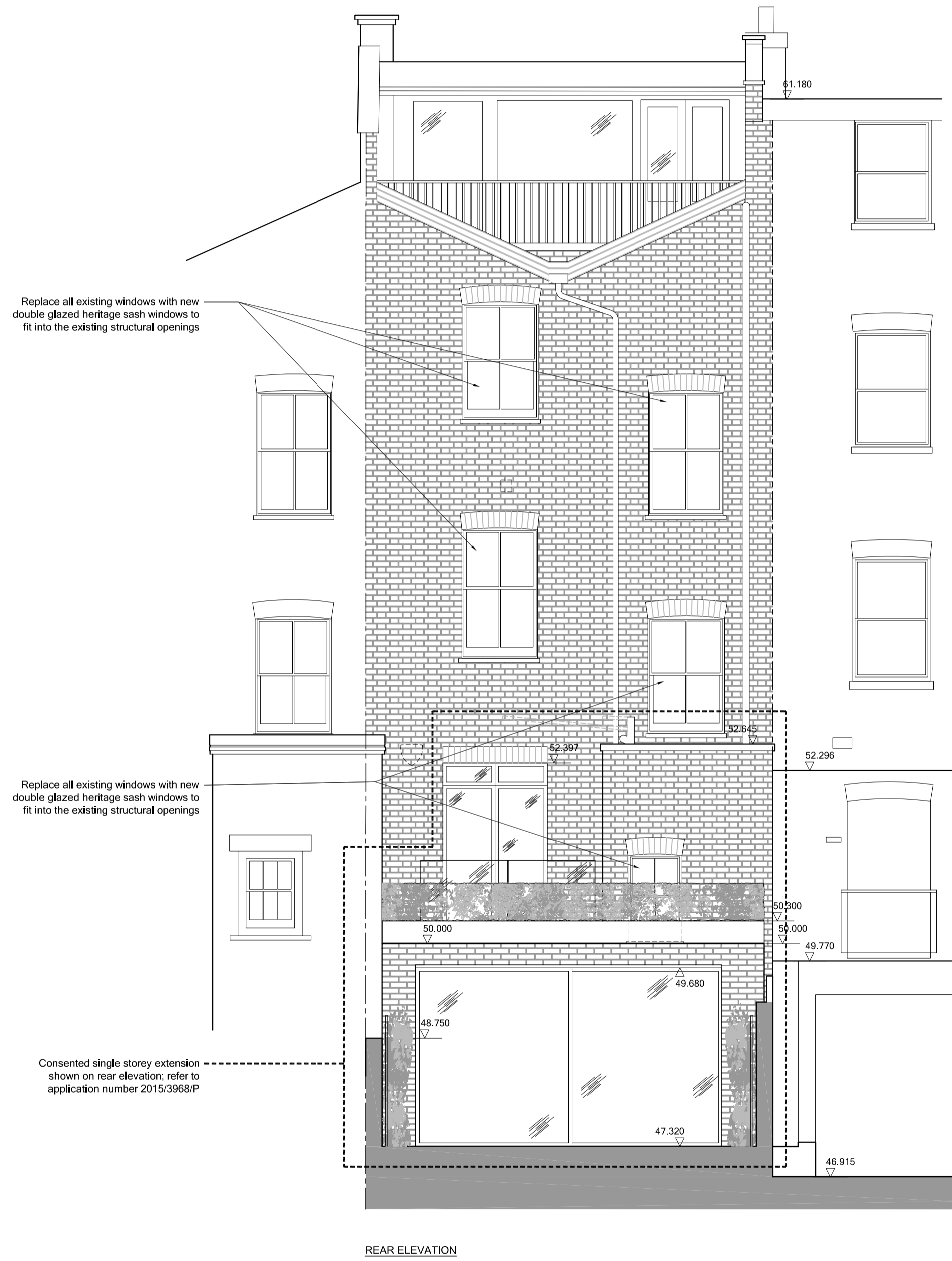
REAR ELEVATION
