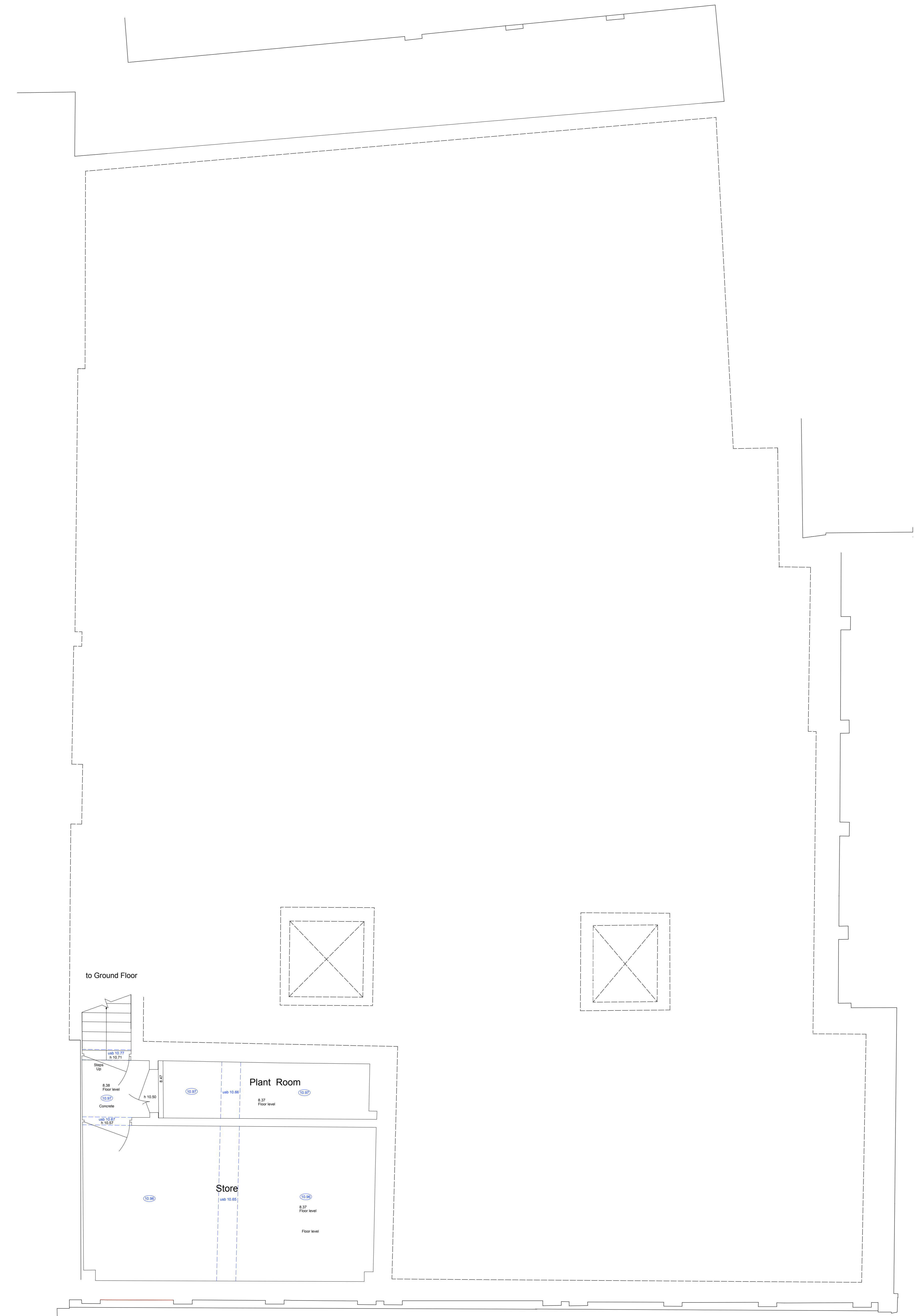
Existing Basement Floor Plan Scale: 1:100 @ A3
