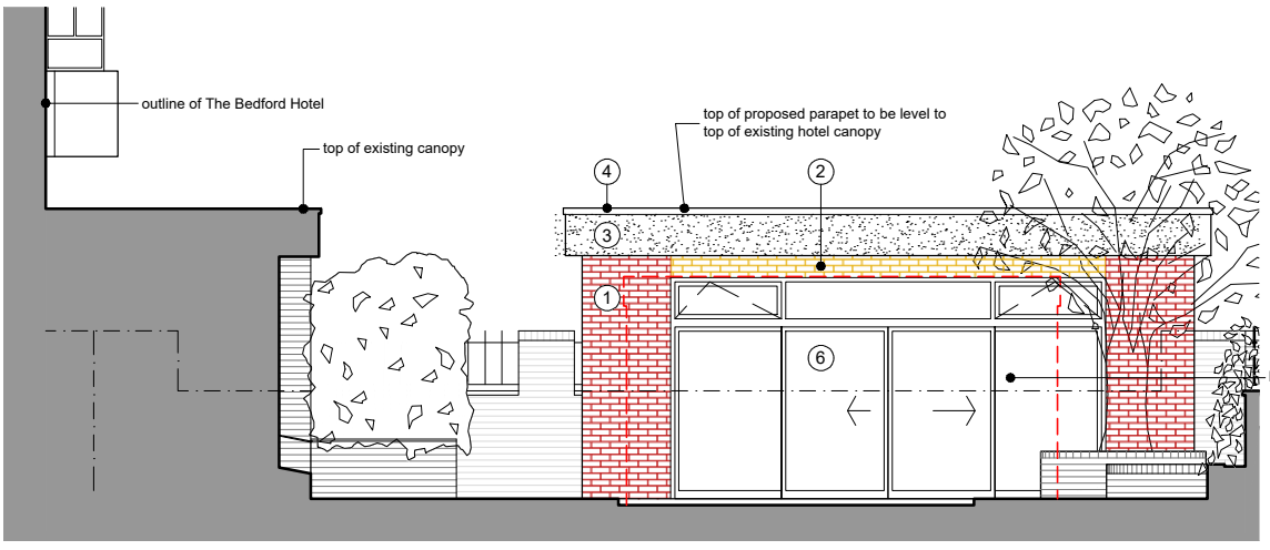
④ FRONT ELEVATION (NW)
