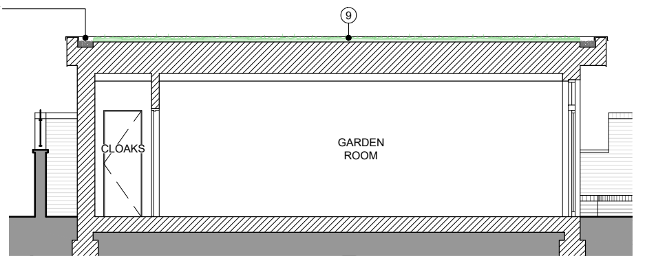
③ LONG SECTION
