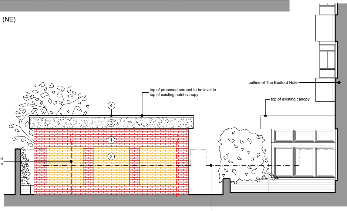
⑥ REAR ELEVATION (SE)
