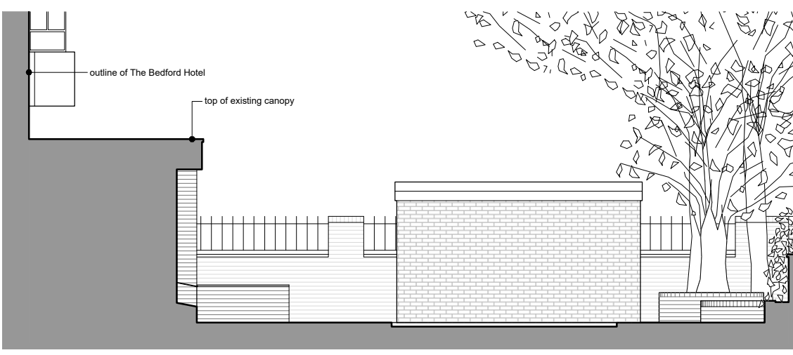
4 FRONT ELEVATION (NW)
