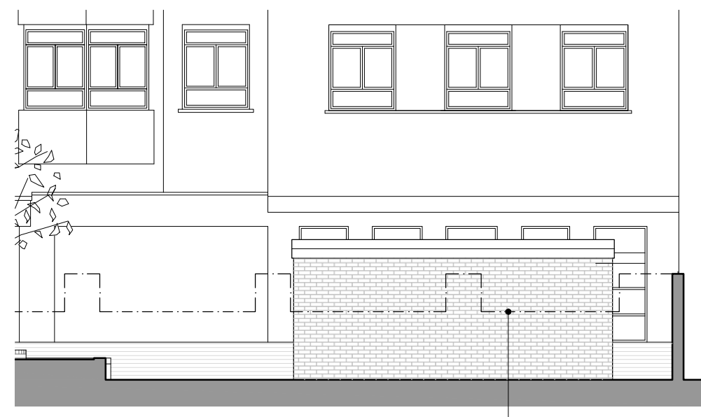
7 SIDE ELEVATION (SW)
