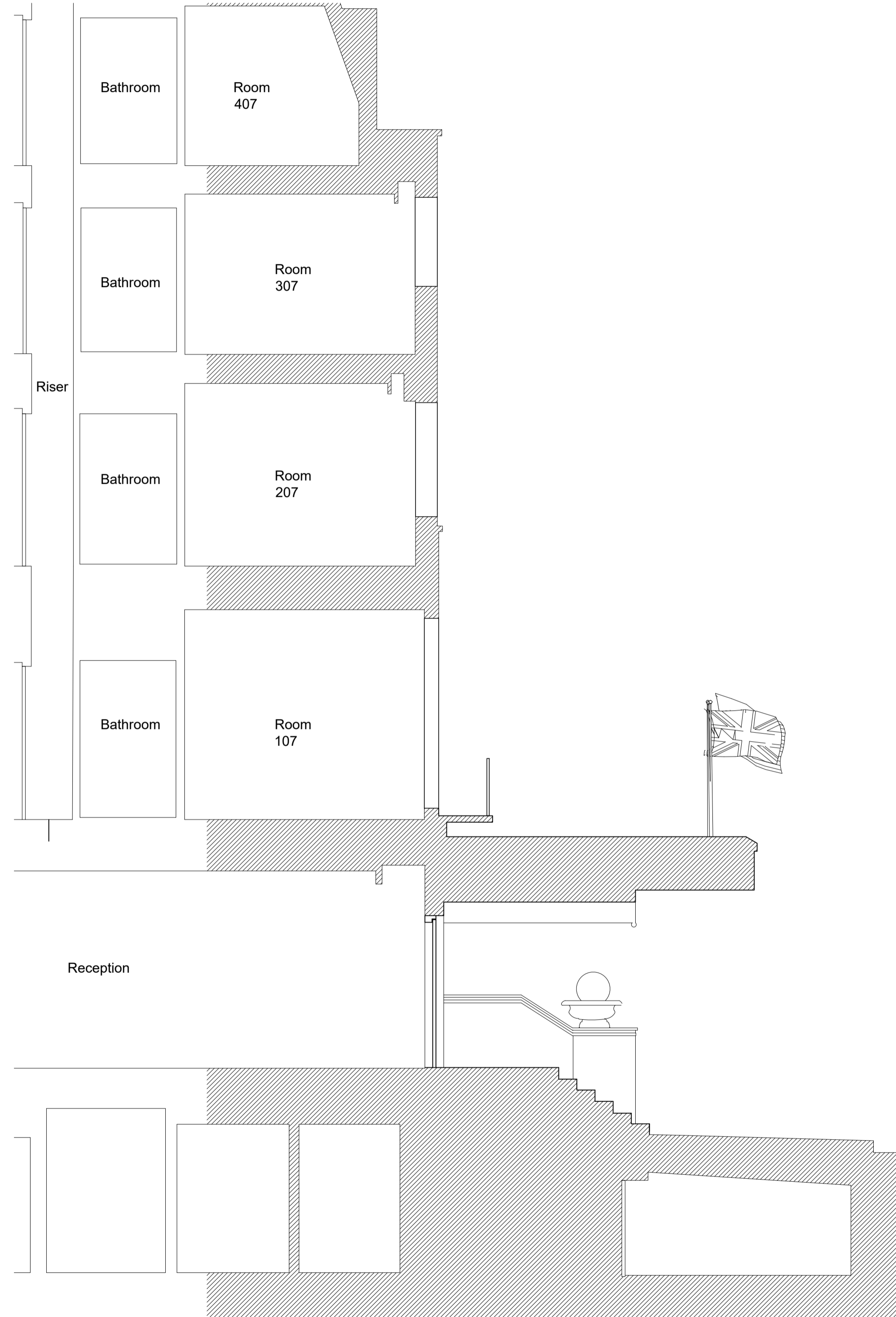
SIDE ELEVATION : AS EXISTING
