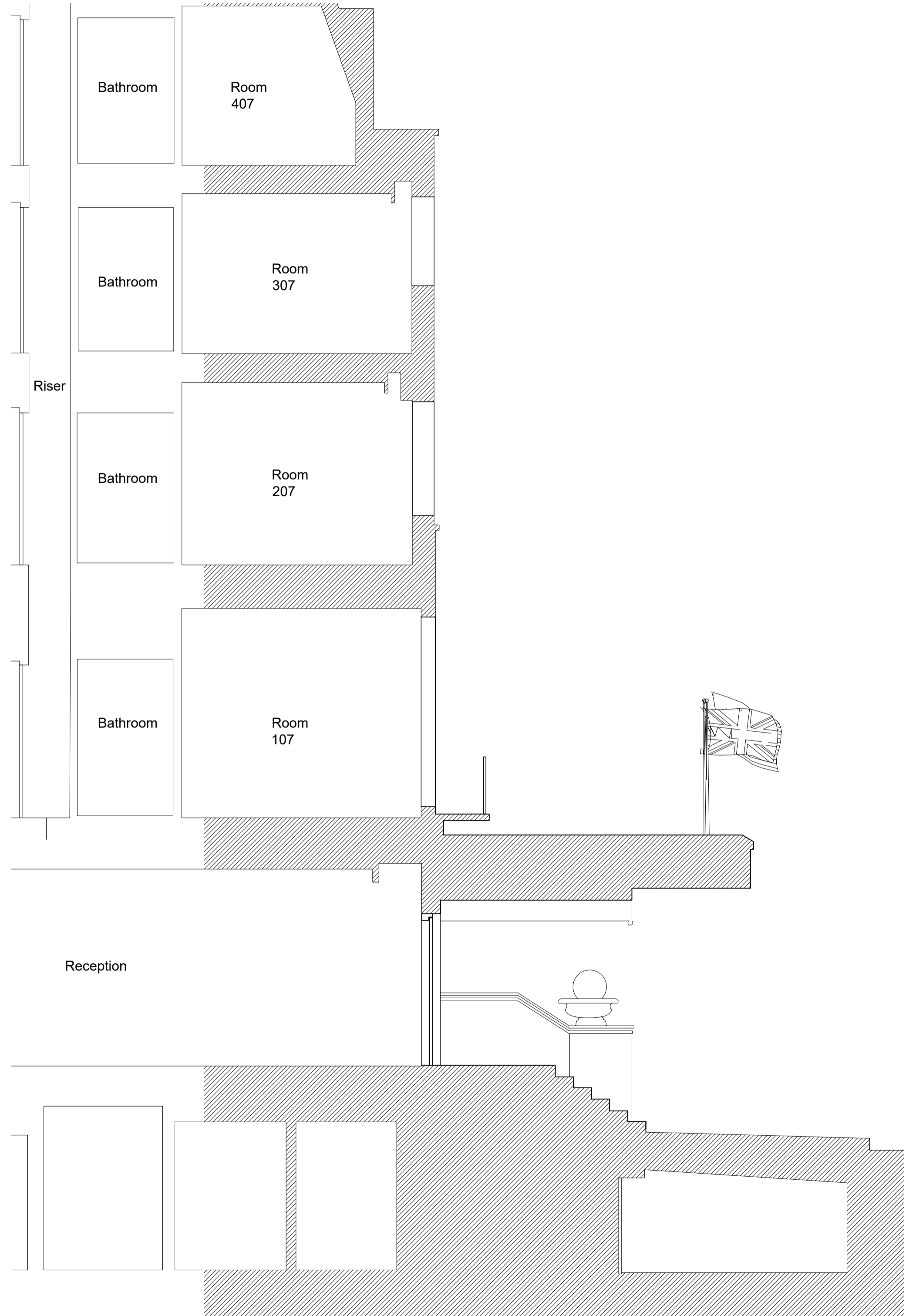
SIDE ELEVATION : AS EXISTING
