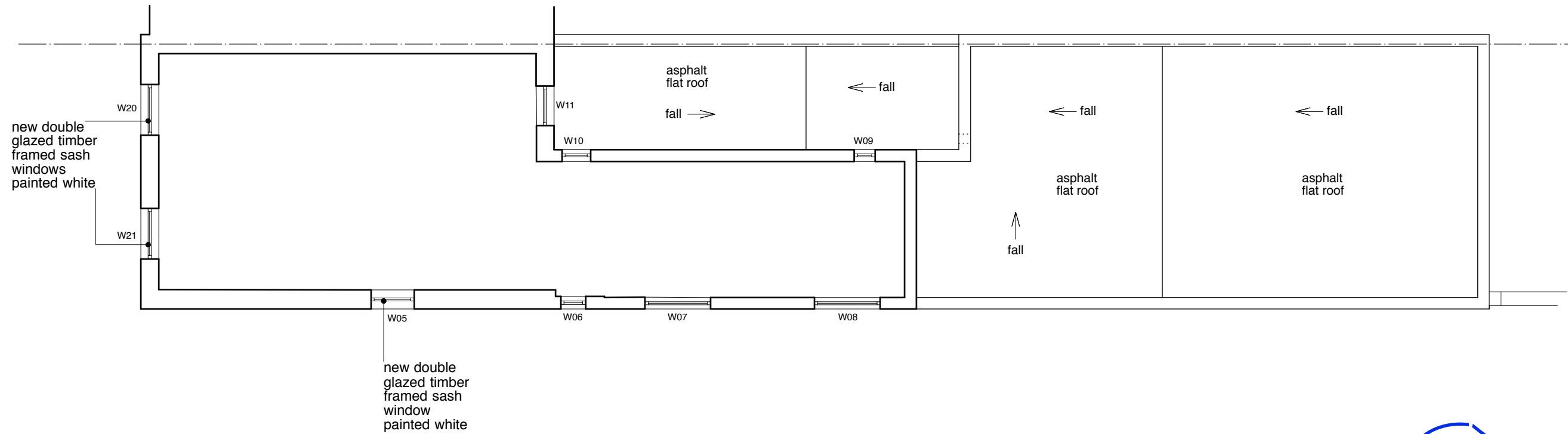
PROPOSED FIRST FLOOR PLAN Scale: 1:100
