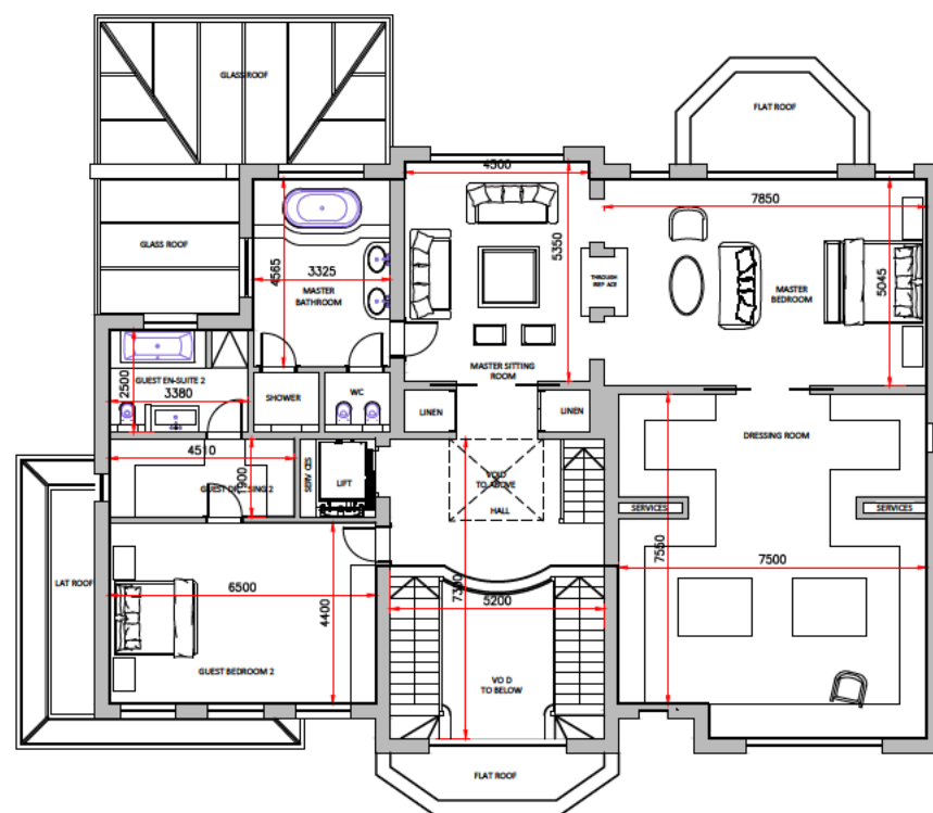
PROPOSED FIRST FLOOR 1:100@A1
