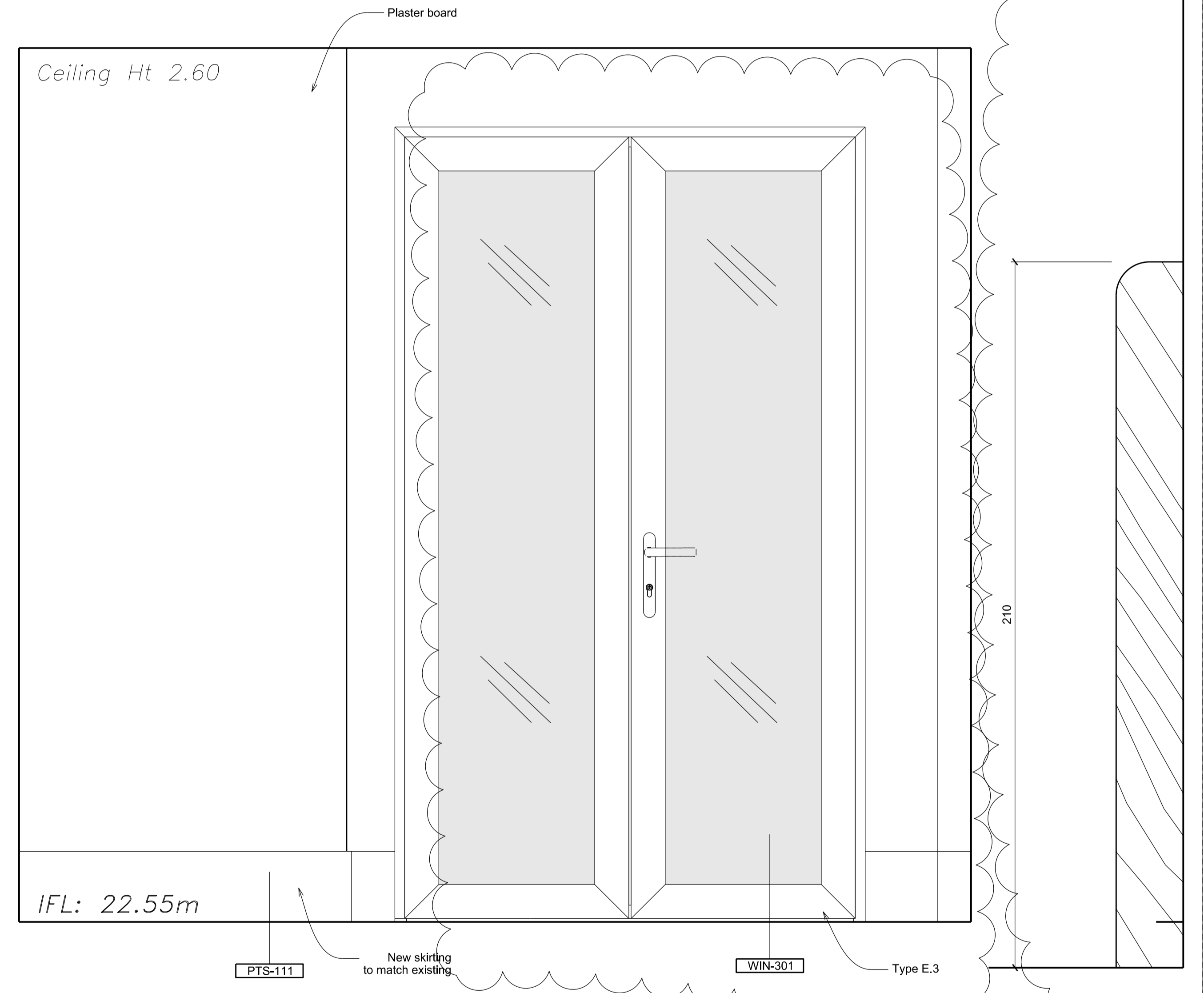
02 Boxing In - Elevation 1:10
