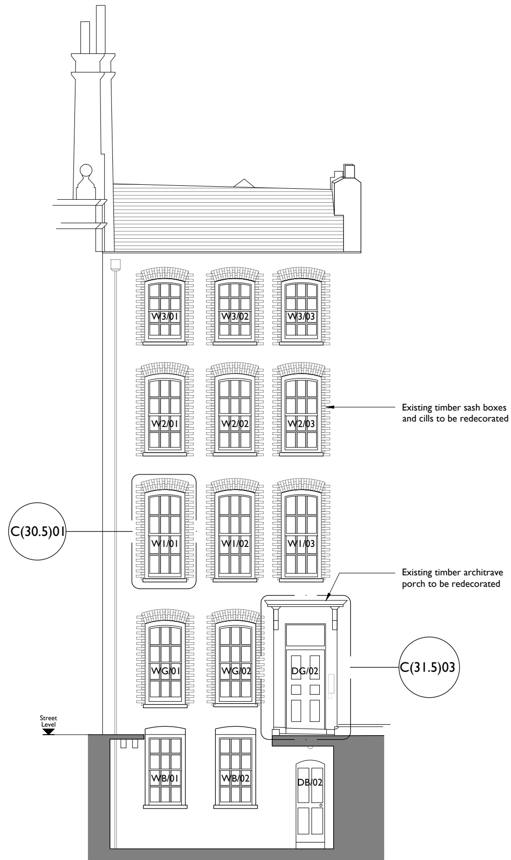
1 Proposed Front Elevation 220 1:100 @ A3
