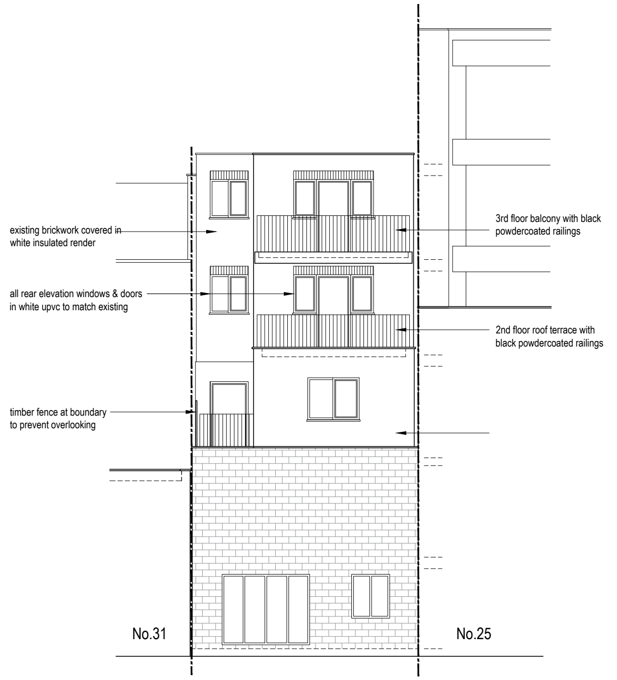
Existing South-West Rear Elevation scale 1:100
