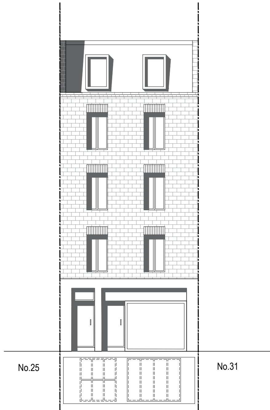
Proposed Front Elevation scale 1:100
