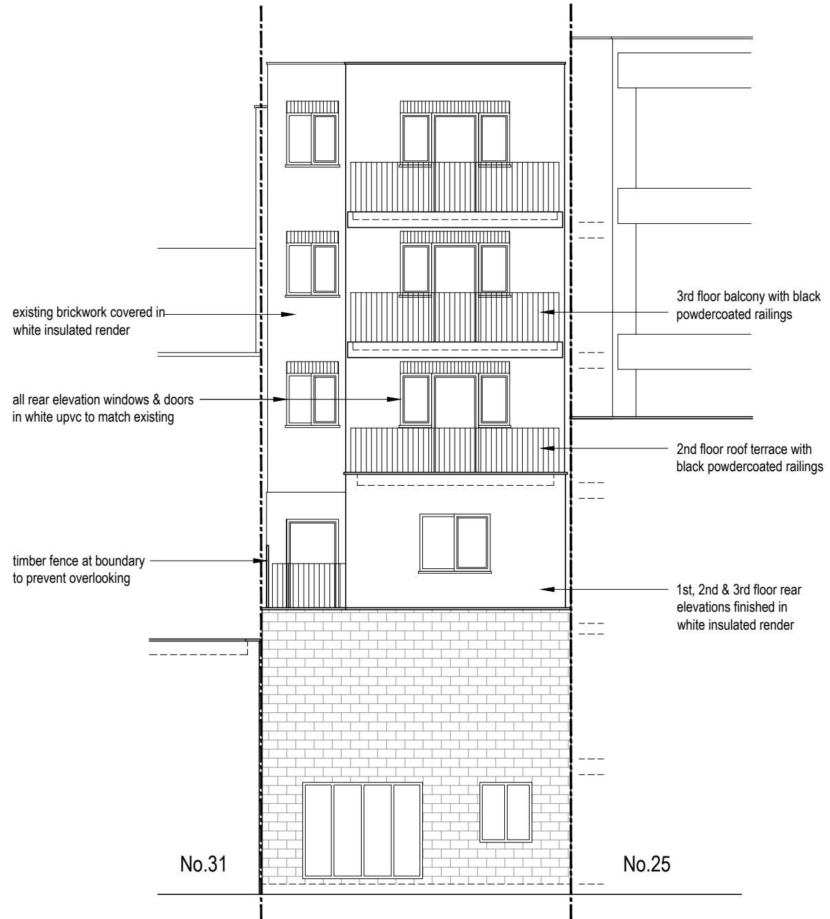
Proposed South-West Rear Elevation scale 1:100
