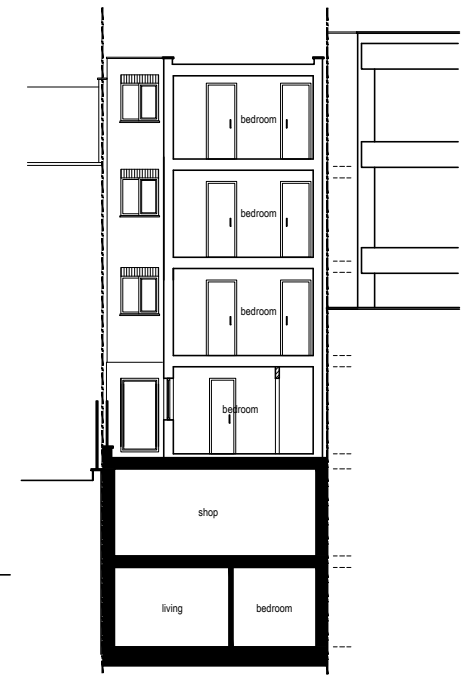
Proposed Section B - B scale 1:200
