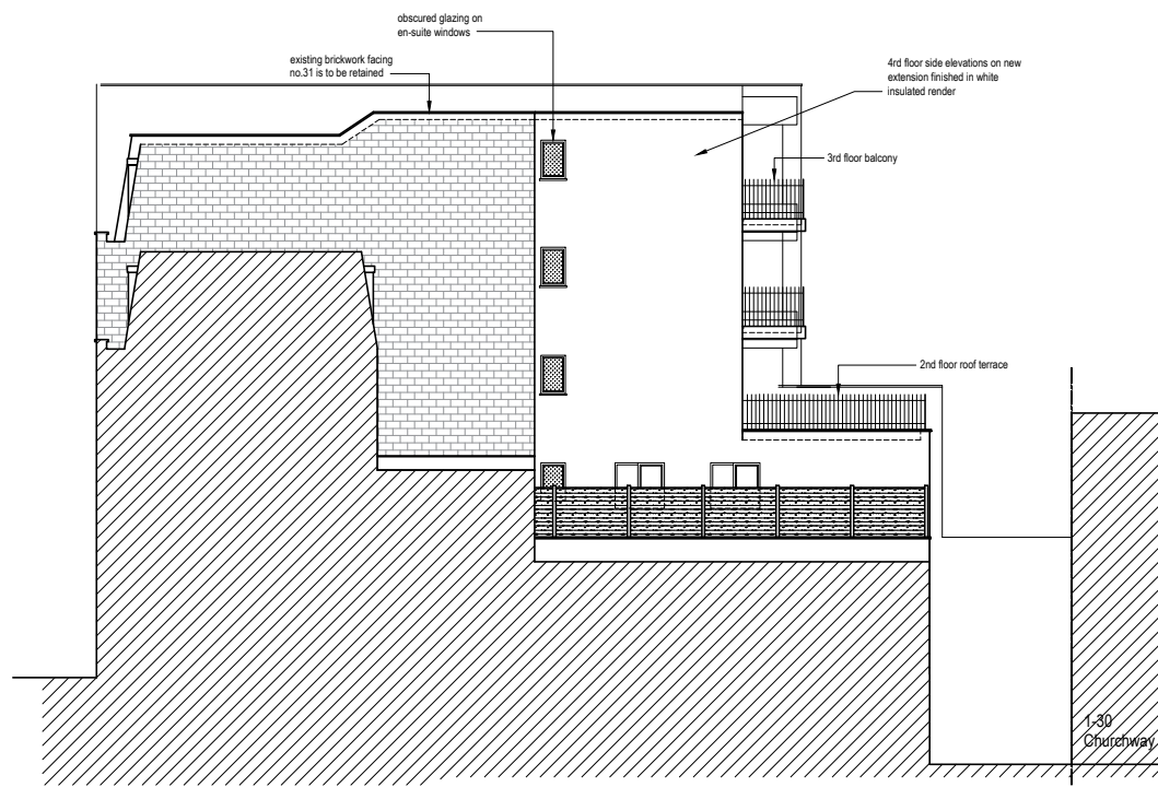
Proposed Side Elevation scale 1:200
