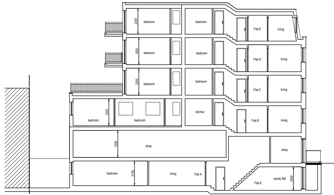
Proposed Section A - A scale 1:200
