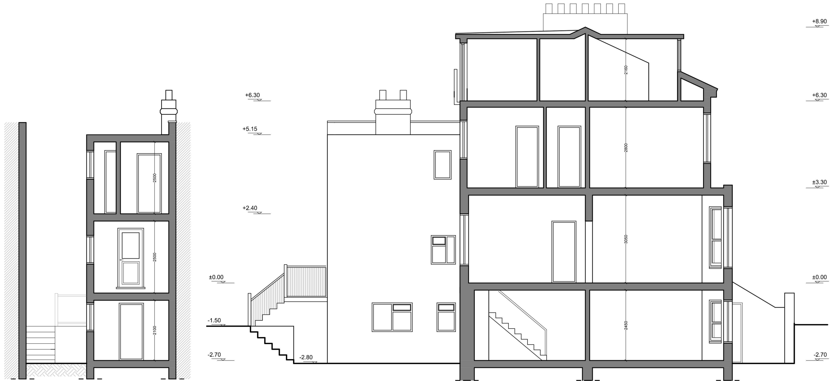
SECTION C-C'
