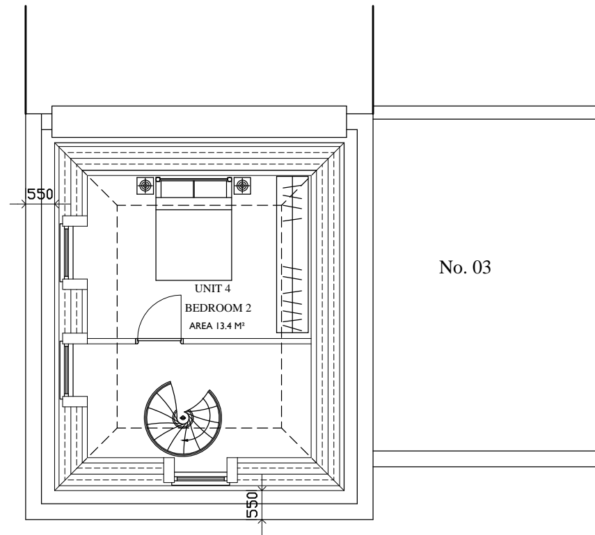
PROPOSED MANSARD ROOF PLAN
