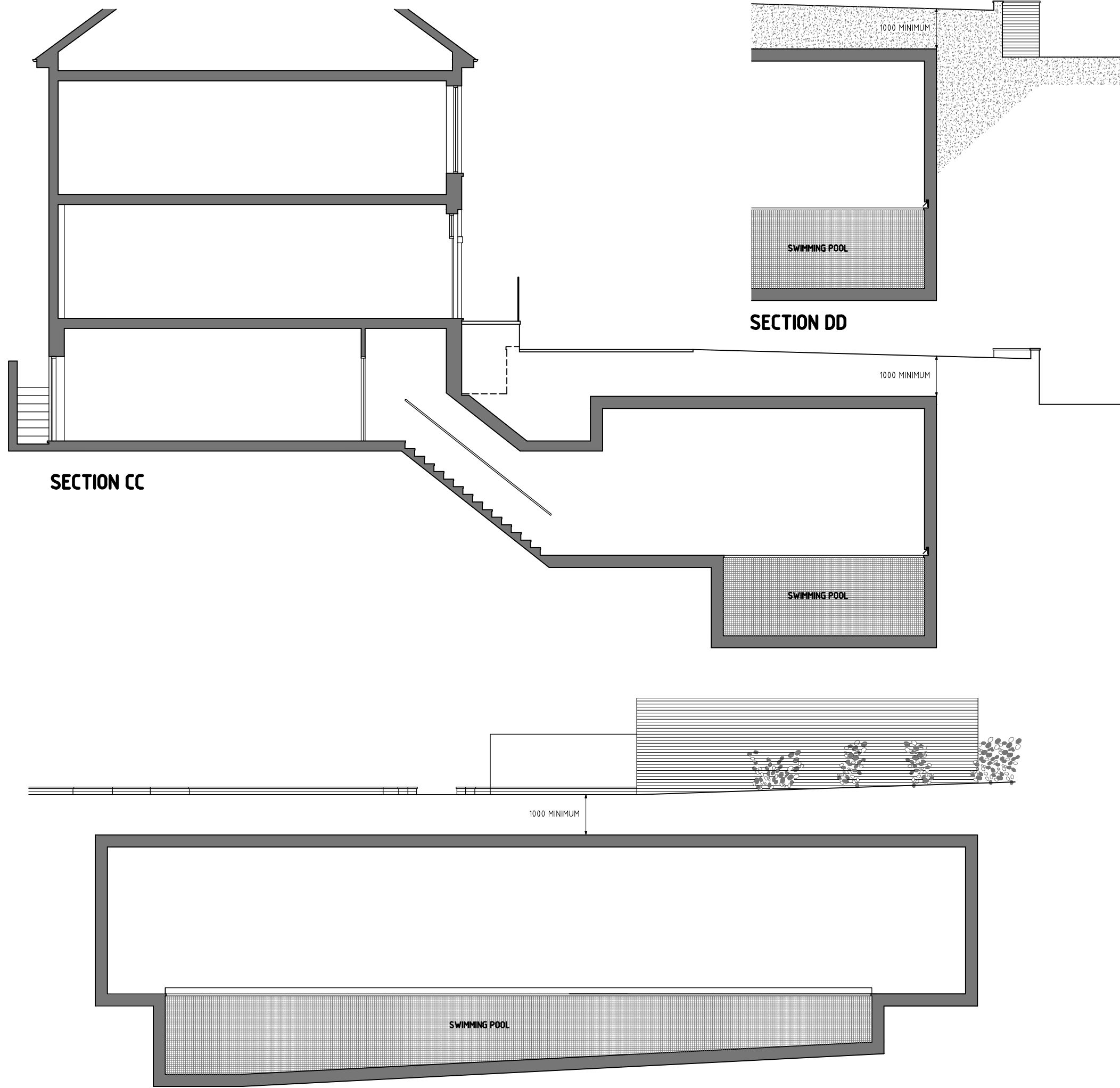
SECTION EE
