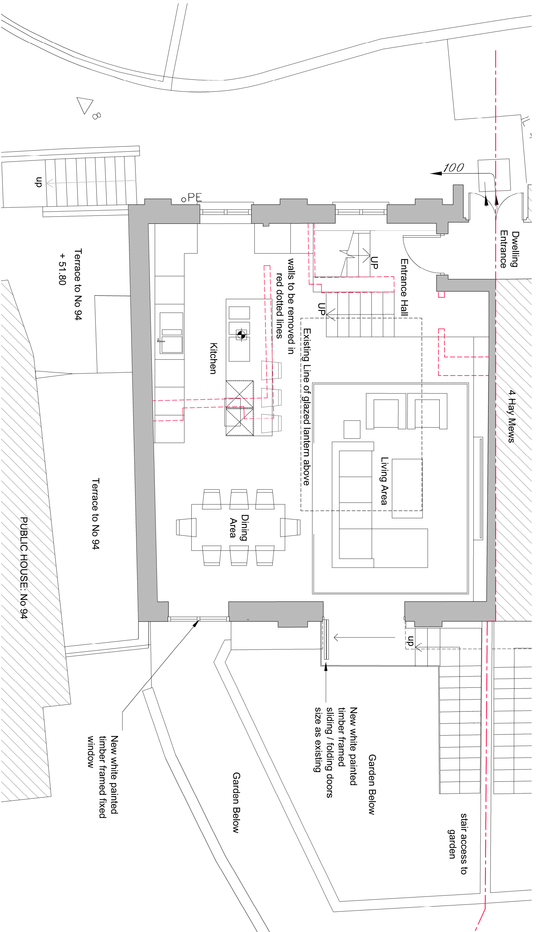
Proposed Upper Ground Floor Plan: 1:50 @ A3
