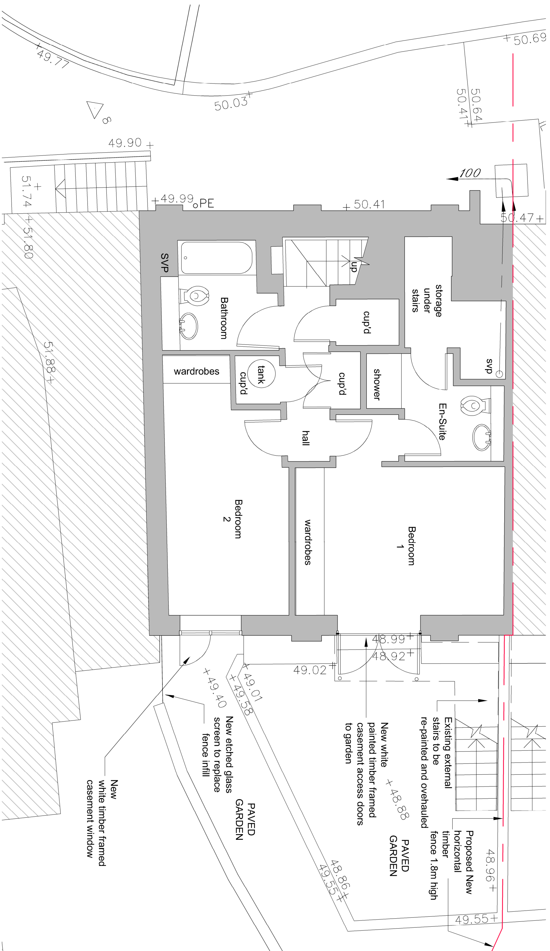
Proposed Lower ground Floor Plan: 1:50 @ A3
