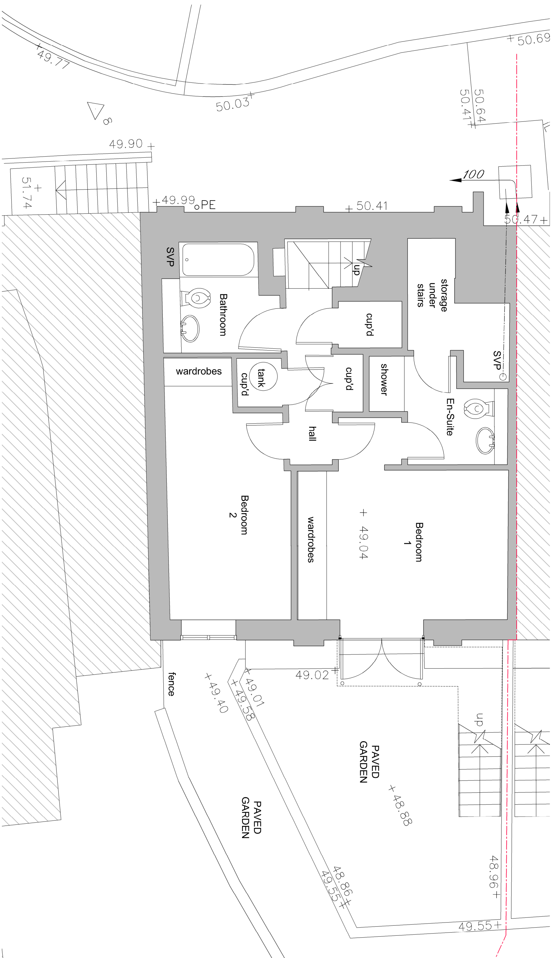
Existing Lower Ground Floor Plan: 1:50 @ A3
