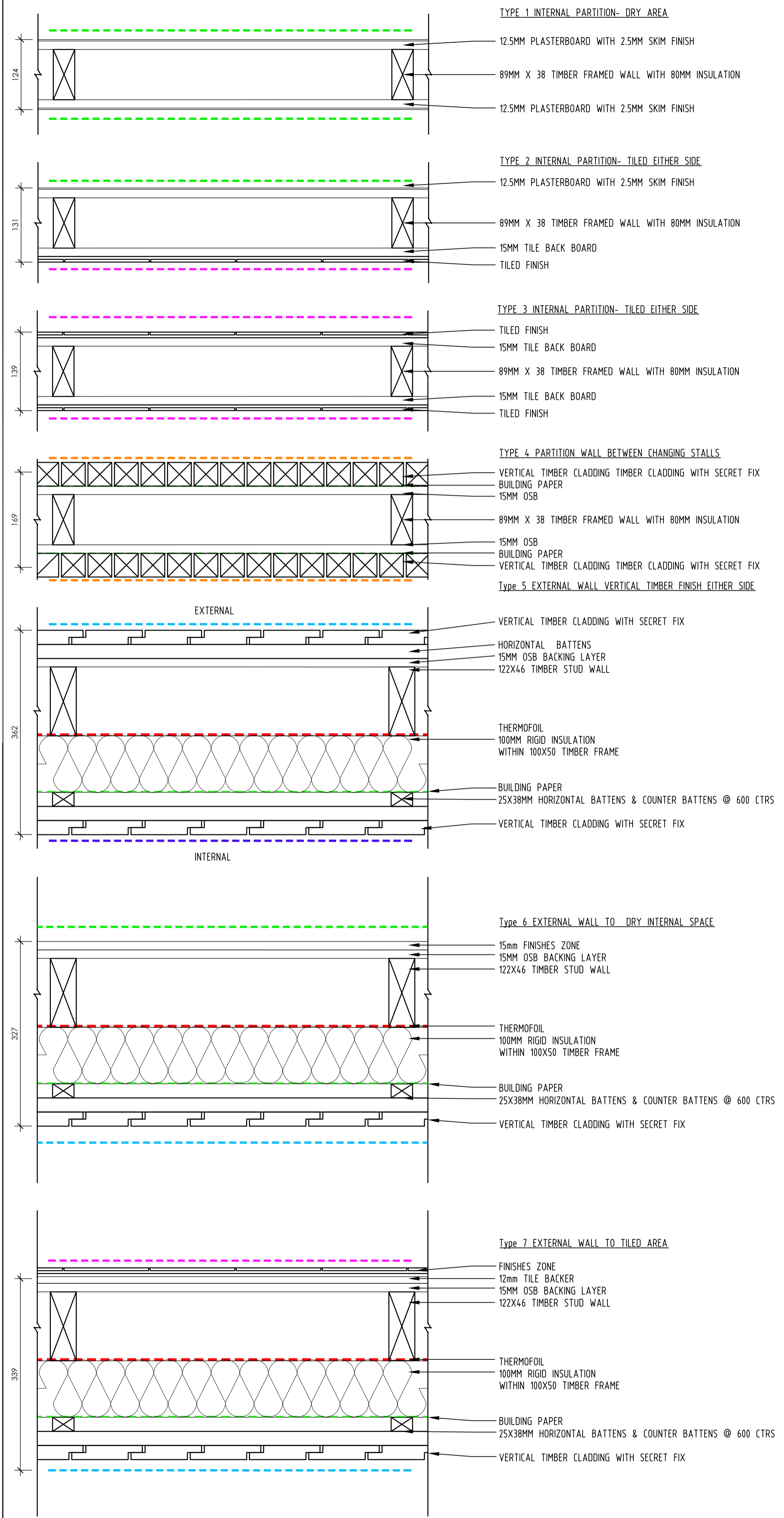
LADIES CHANGING UNIT SCALE 1:50
