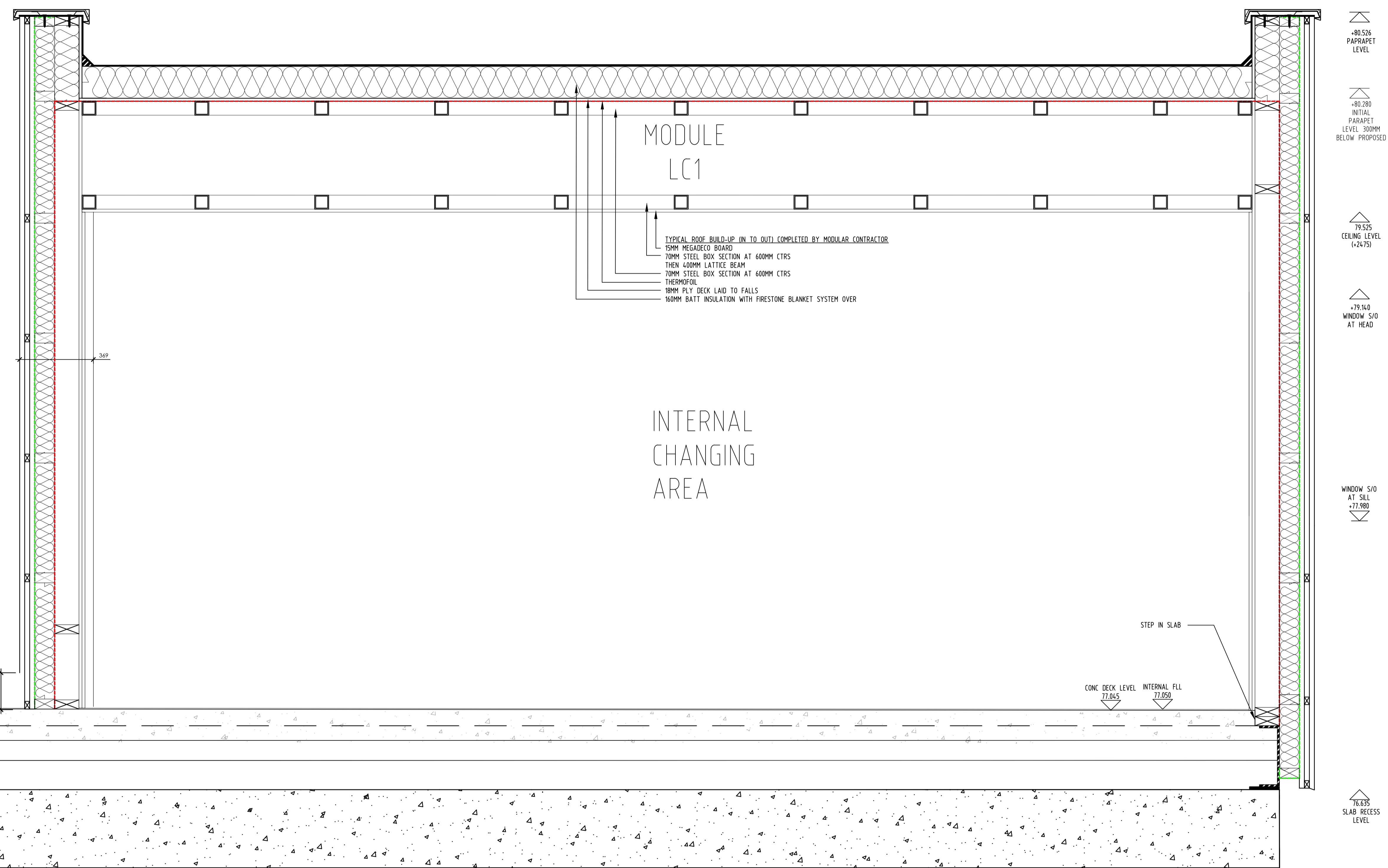
SECTION D-D SCALE 1:10
