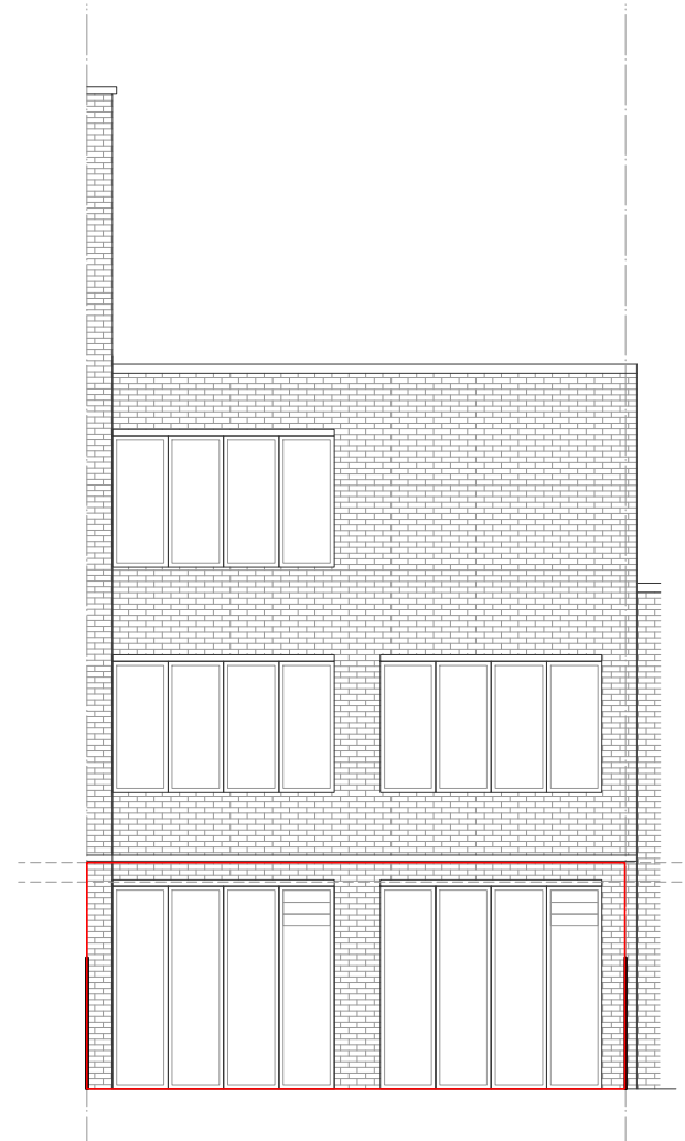
REAR ELEVATION E:1/100
