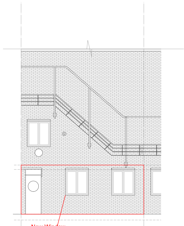
FRONT ELEVATION E:1/100
