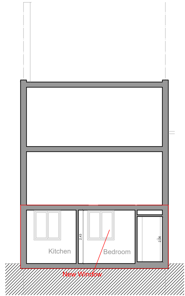
SECTION A-A' E:1/100
