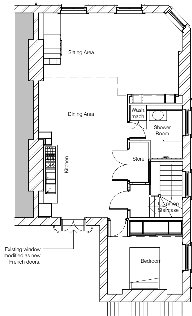
1 | Level 3 - Proposed 1 : 100
