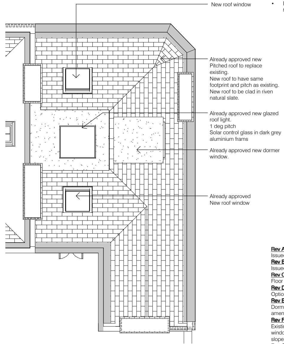
3 | Roof - Proposed 1 : 100
