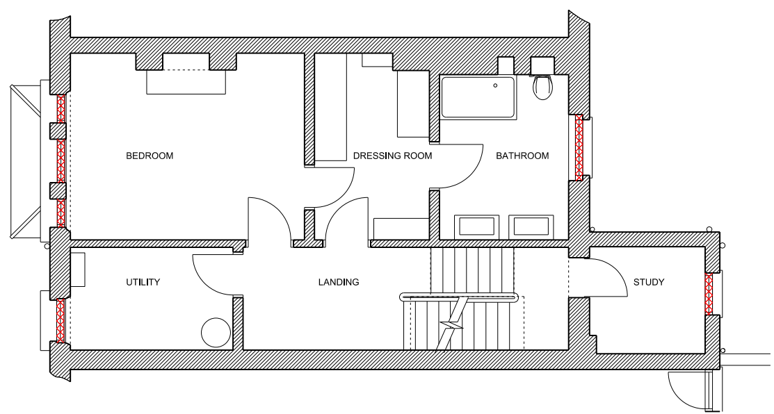
1 1:50 AT A1 EXISTING FIRST FLOOR PLAN
