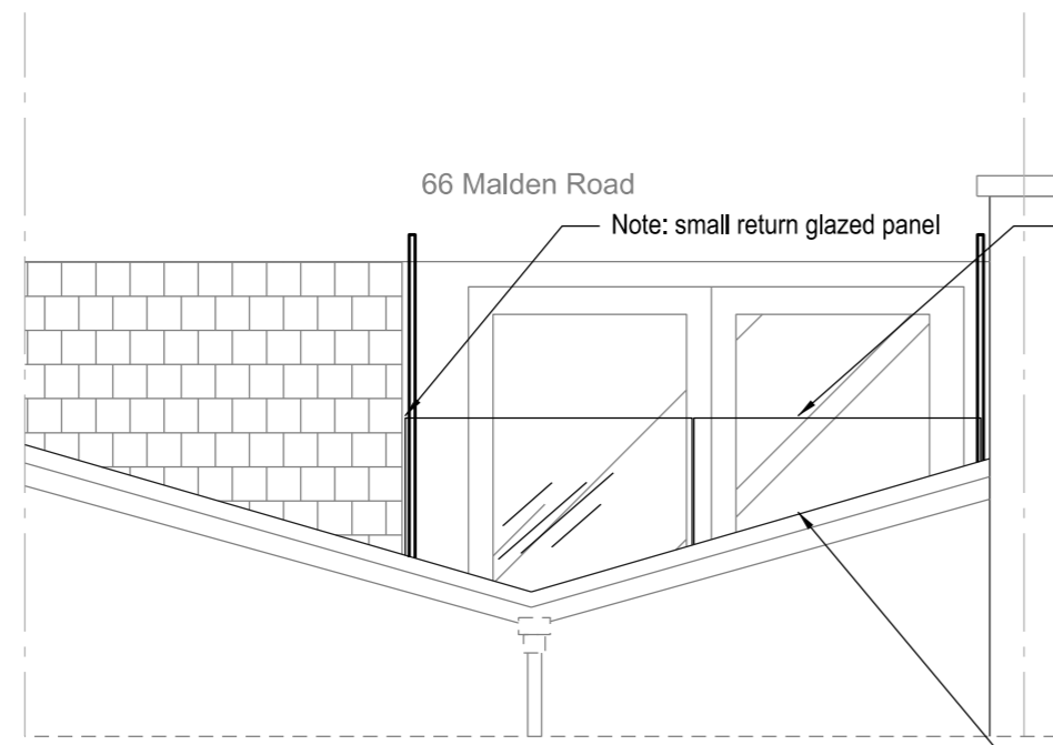
Detail Elevation 1
