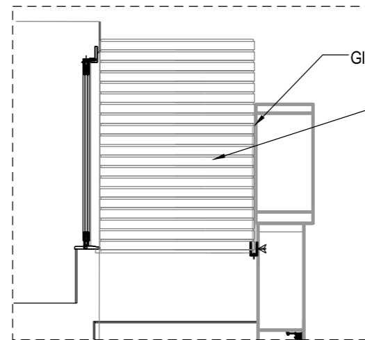
Detail Elevation 4
