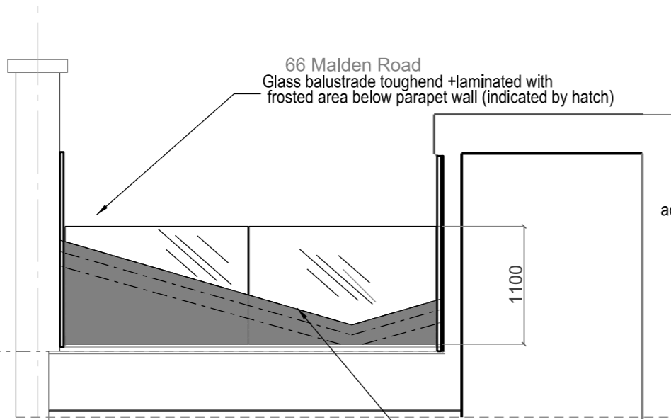
Detail Elevation 2
