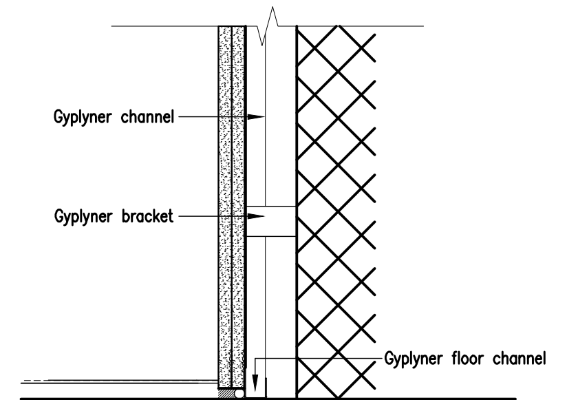
DETAIL 6 WALL LINING BASE DETAIL (TYPE L1) SCALE: 1:5
