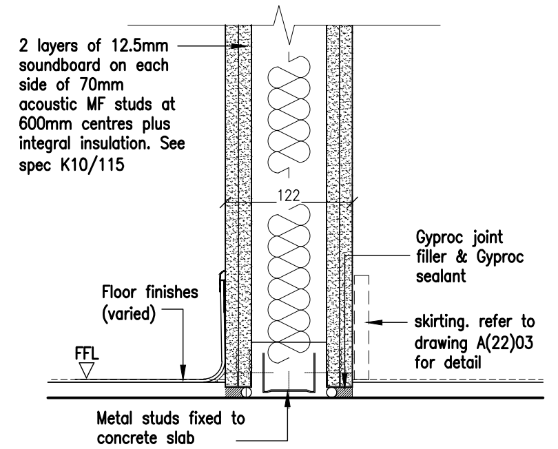
DETAIL 3 PLASTERBOARD PARTITION BASE DETAIL SCALE: 1:5
