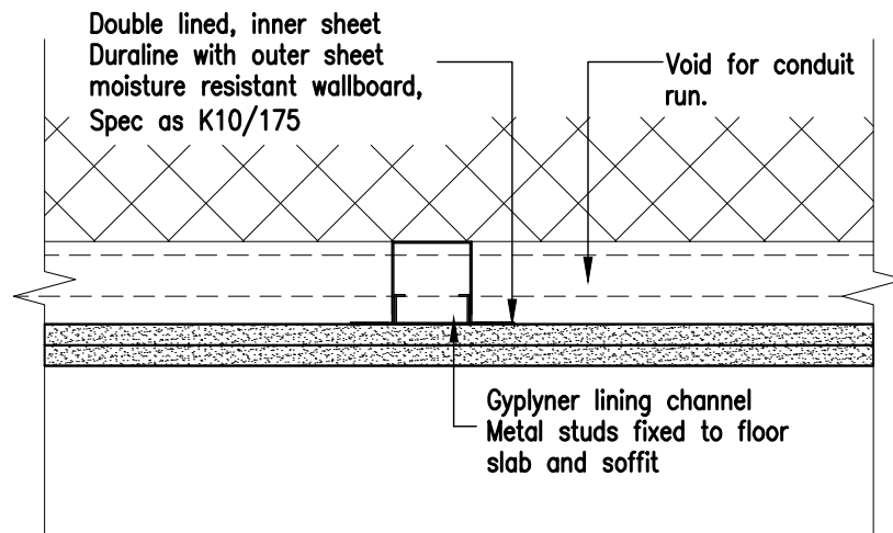
DETAIL 4 WALL LINING (TYPE L1) SCALE: 1:5
