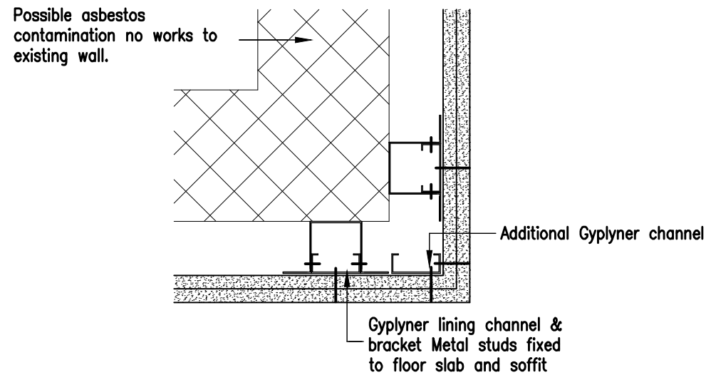
DETAIL 5 WALL LINING CORNER (TYPE L1) SCALE: 1:5
