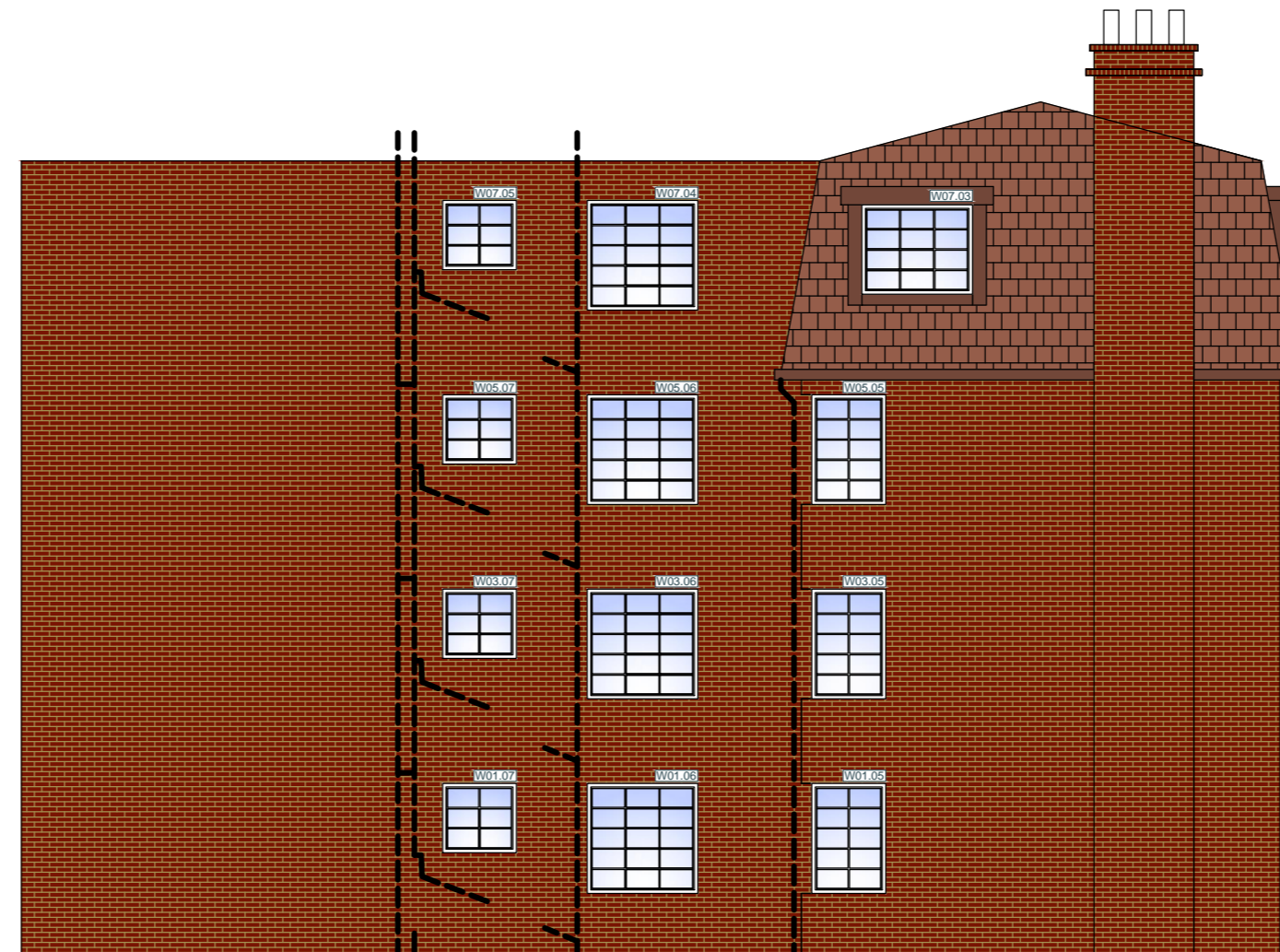
ELEVATION E-E
