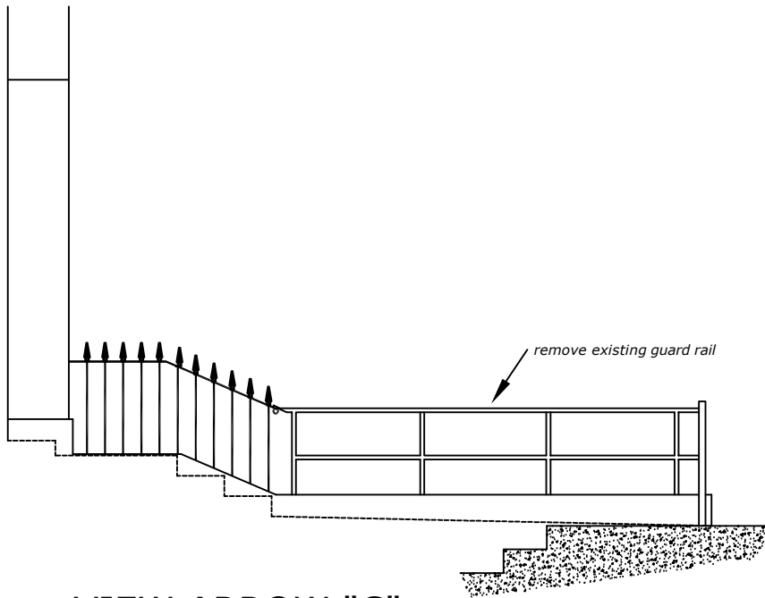
VIEW ARROW "C" [EXISTING]
