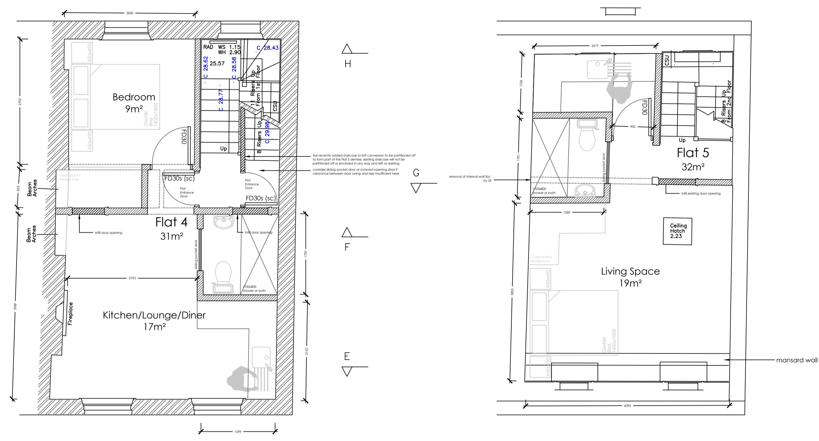
16 PROPOSED SECOND FLOOR PLAN 1:50
