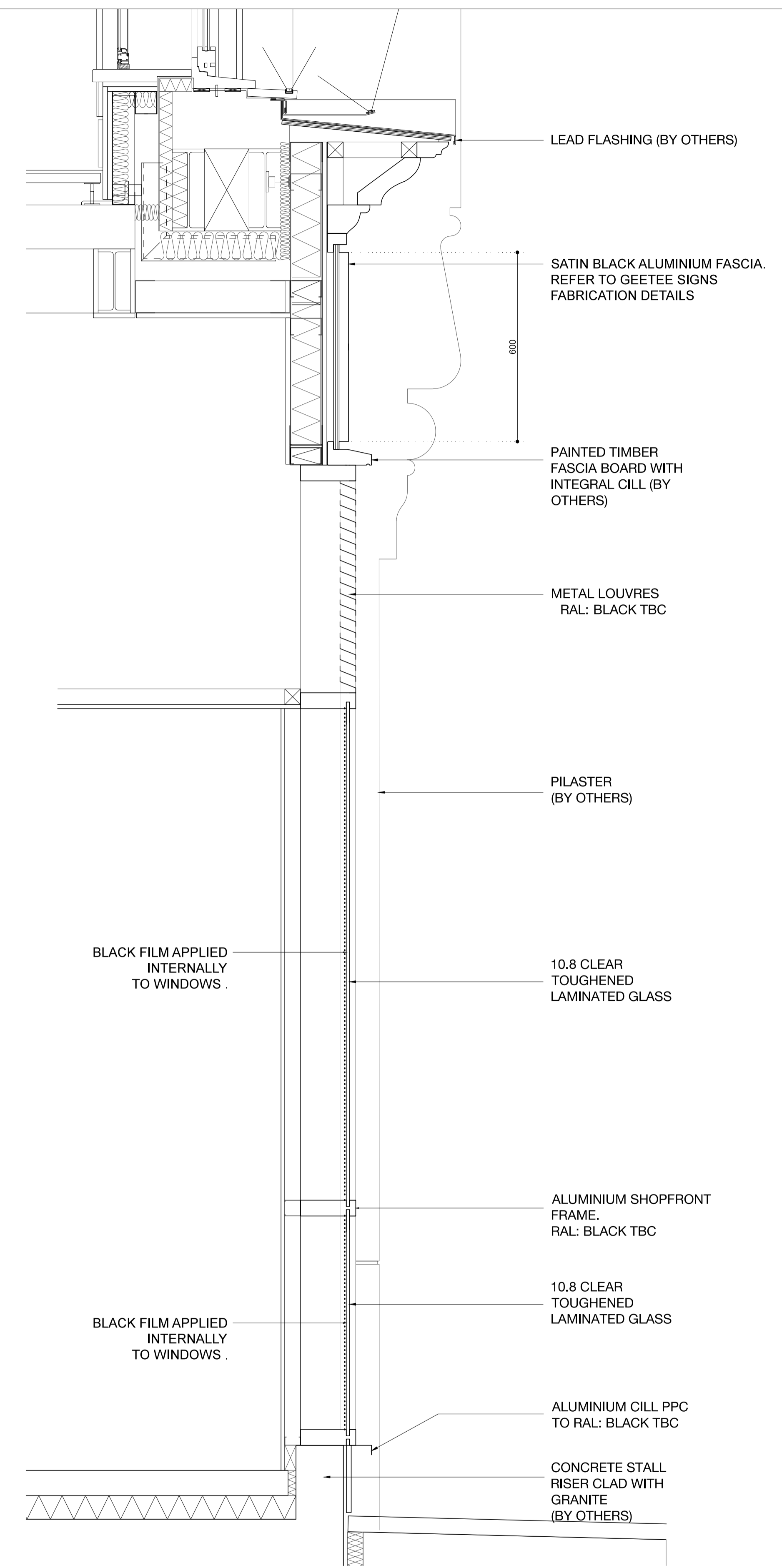
03 SECTION THRU LOUVRES SCALE 1:10 @ A1
