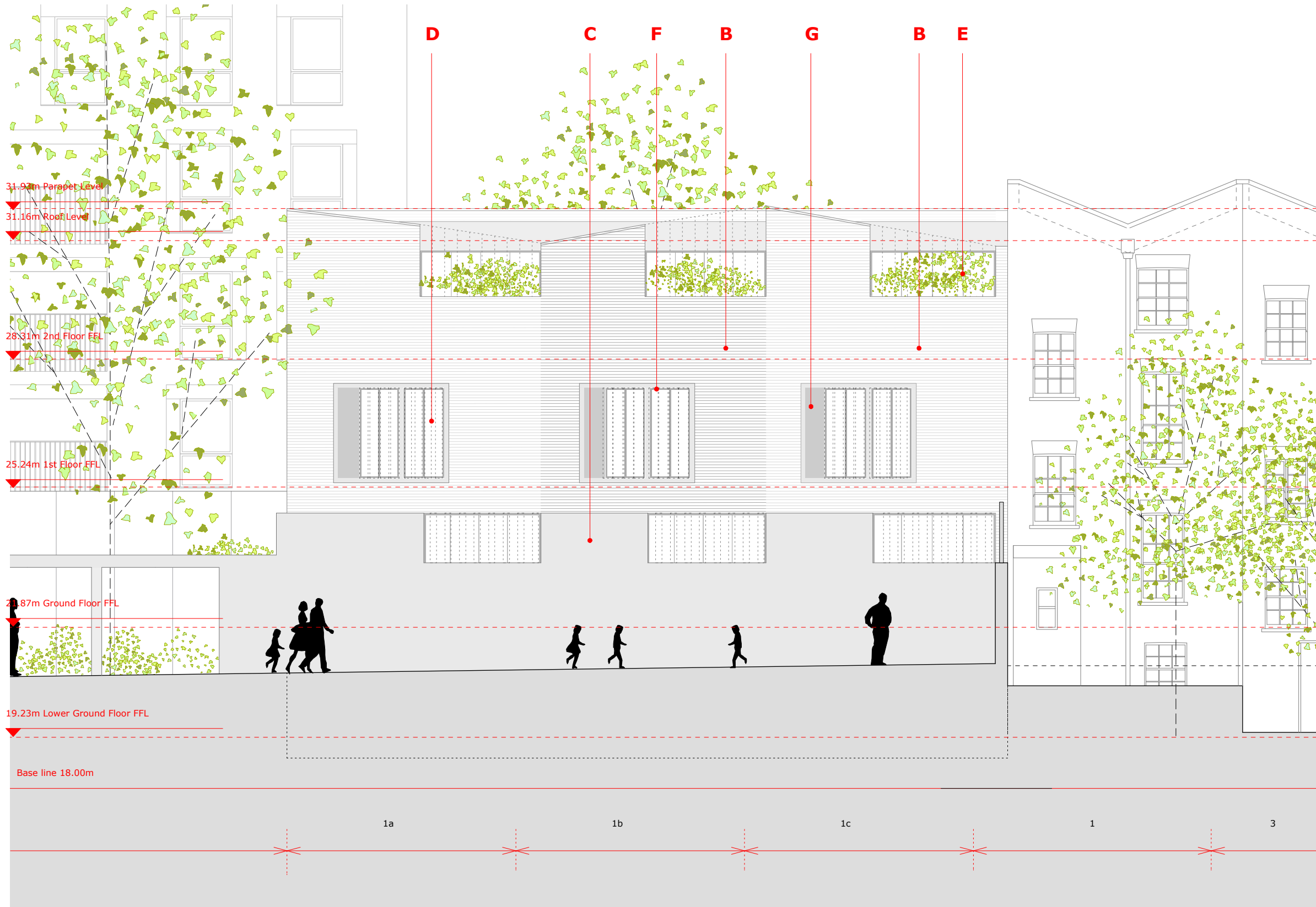
North East Elevation, Rear of Charrington Street 1:100
