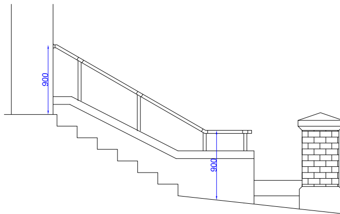
Proposed side elevation - Steps
