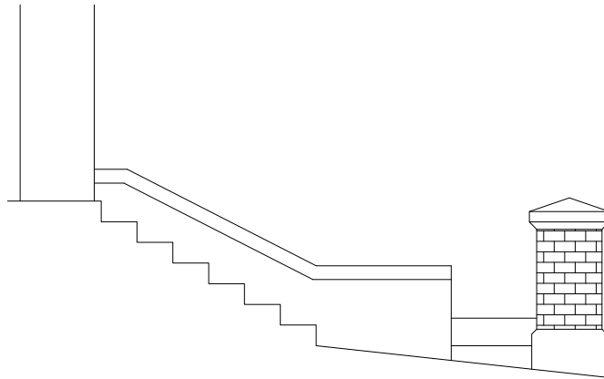
Existing side elevation - Steps
