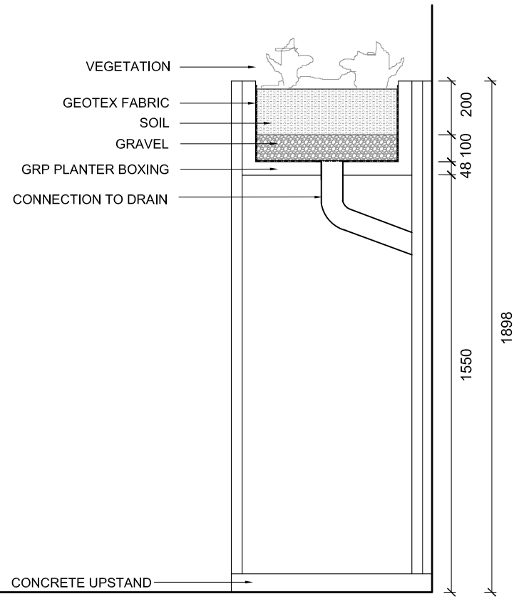
SECTION A
