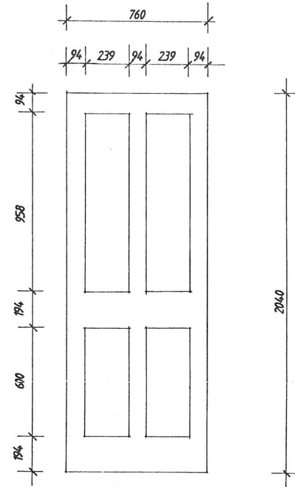
DOOR NOS. D F03, D S01, D S02, D S03, D S04.
