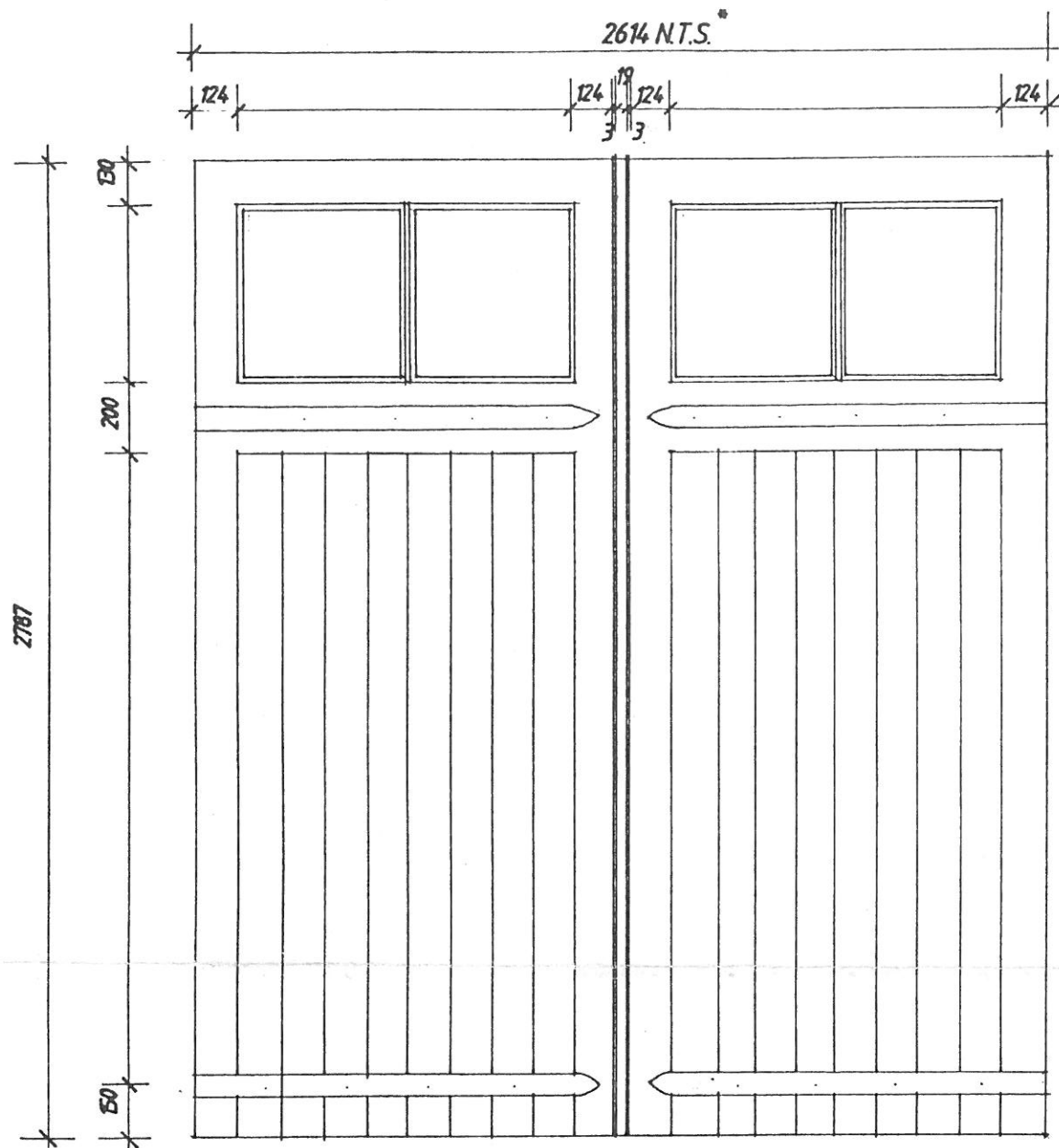
DOOR NO D G02. * Exact door leaf sizes to be agreed onsite.
