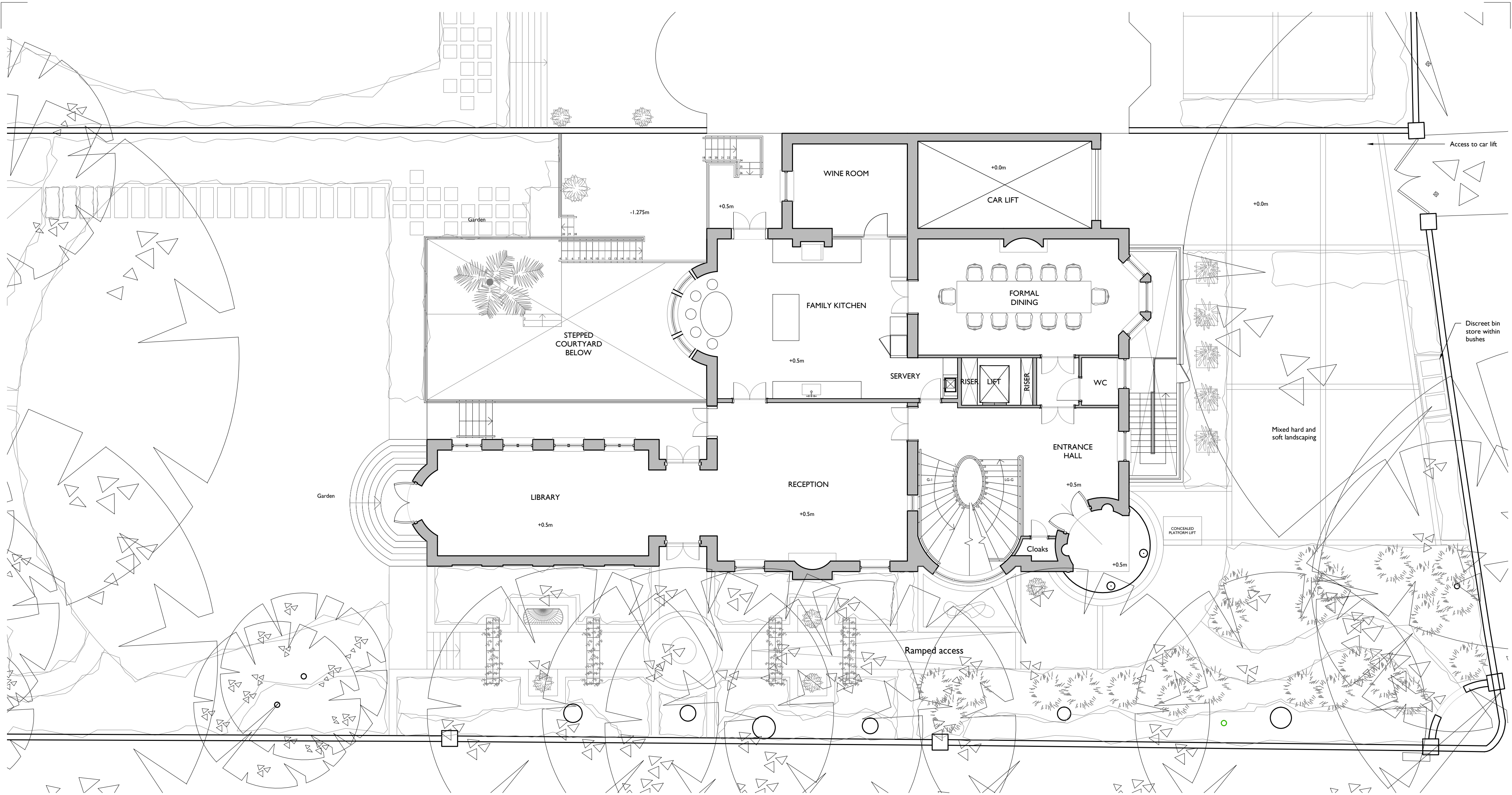
I 73 Proposed Ground Floor Plan 202 I:100@A2
