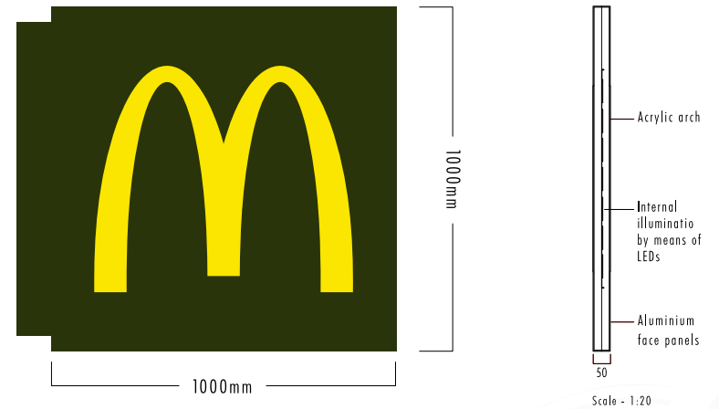
LIM 10 1000mm x 1000mm LED ILLUMINATED DOUBLE SIDED PROJECTING SIGN scale 1:20
