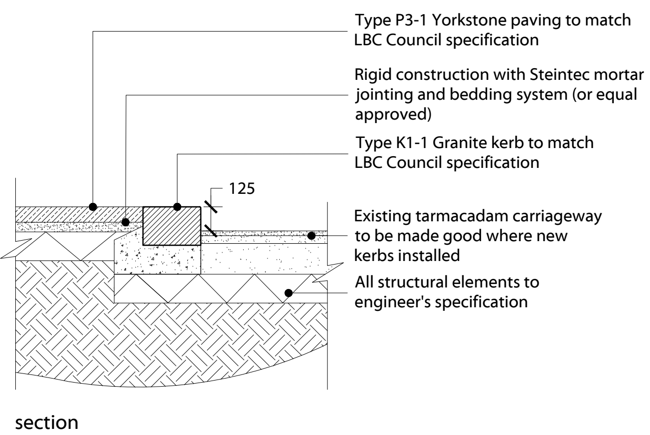
B Typical details of West End Lane paving 601 SECTION 1:20 @ A1
