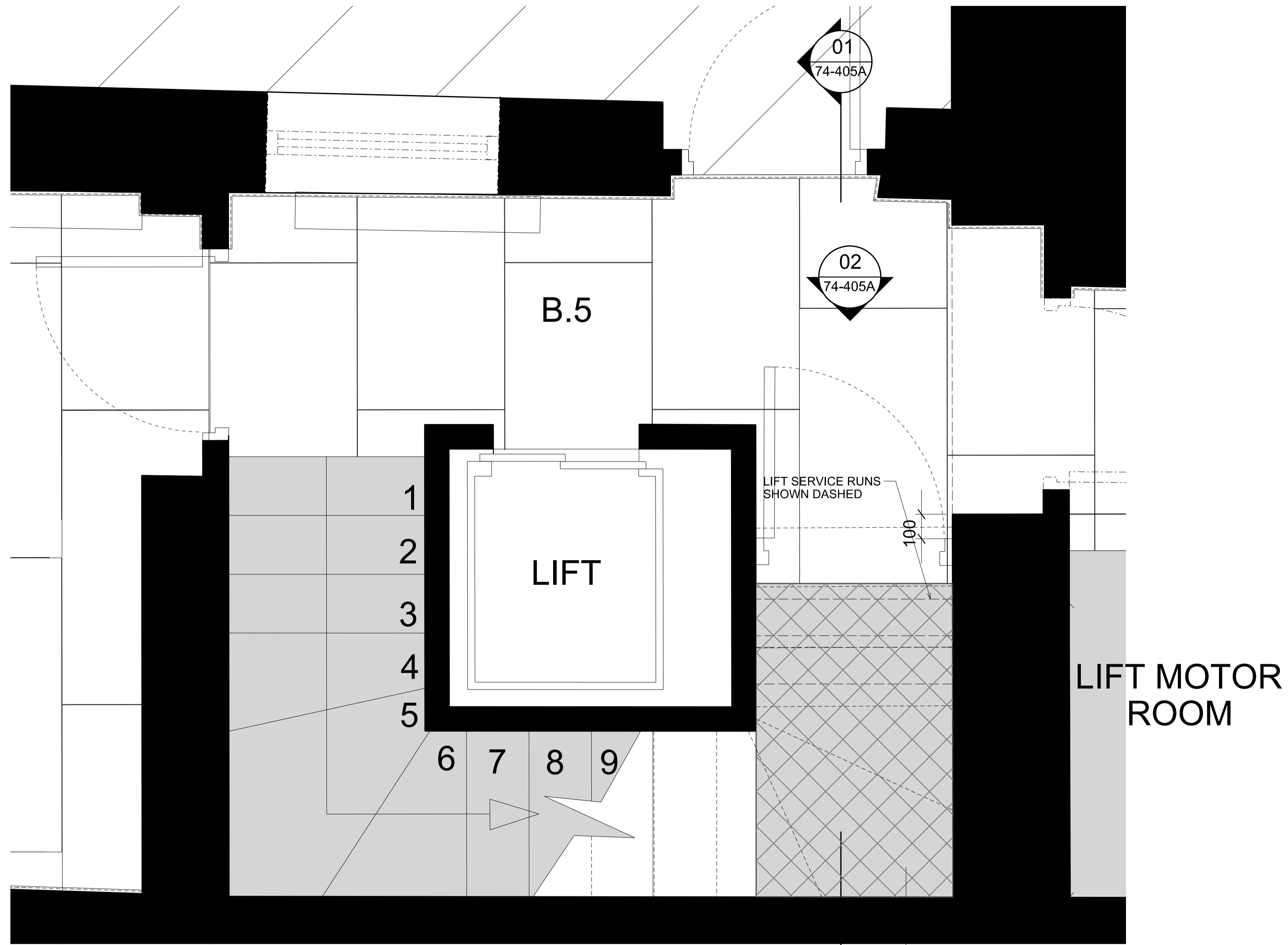
01 LOWER GROUND STAIR PLAN 1:10
