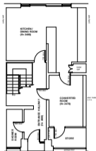
EXISTING GROUND FLOOR PLAN
