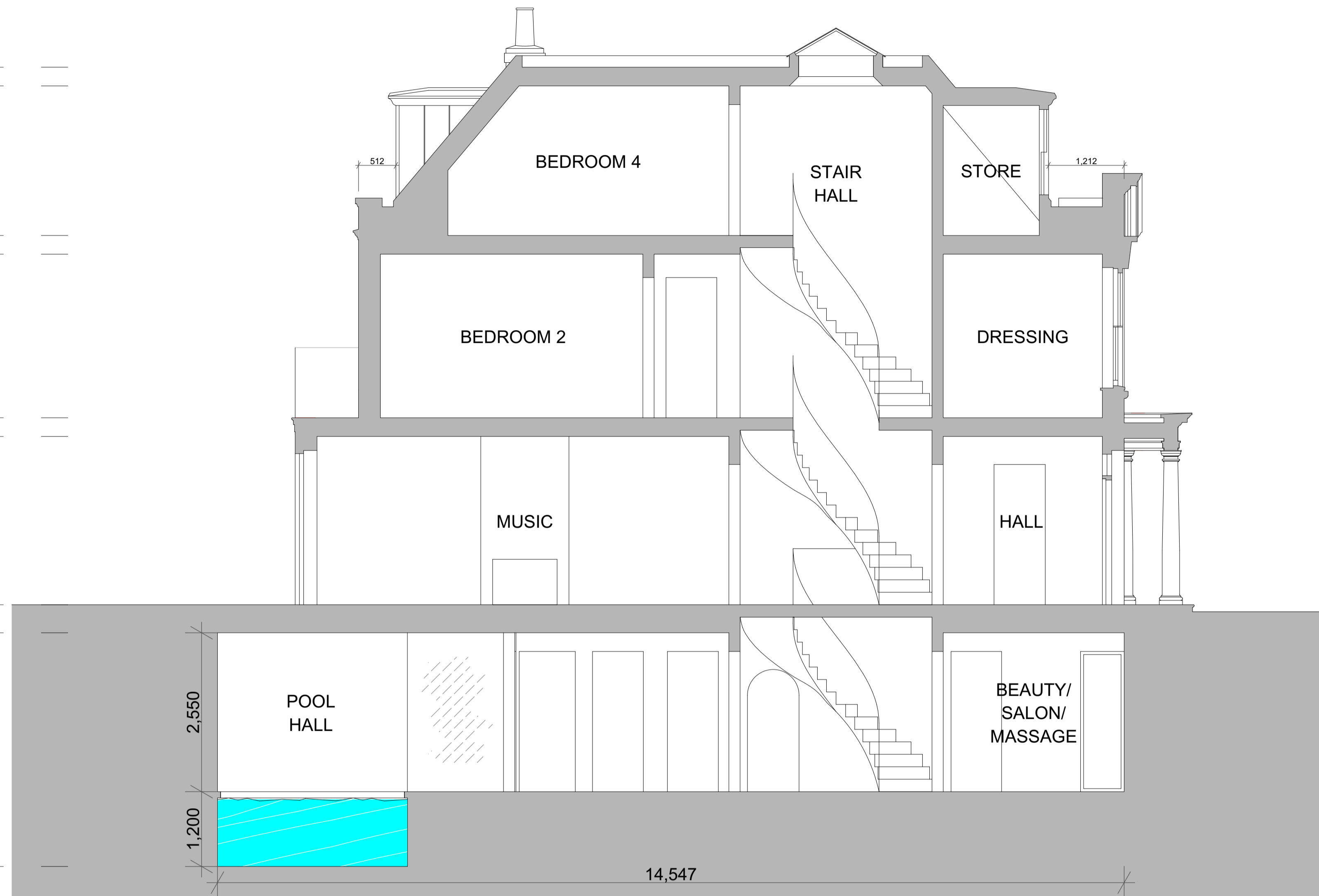
LONG SECTION
