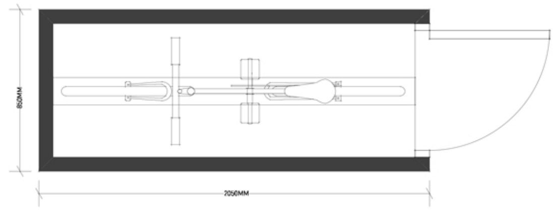
FLOOR PLAN
