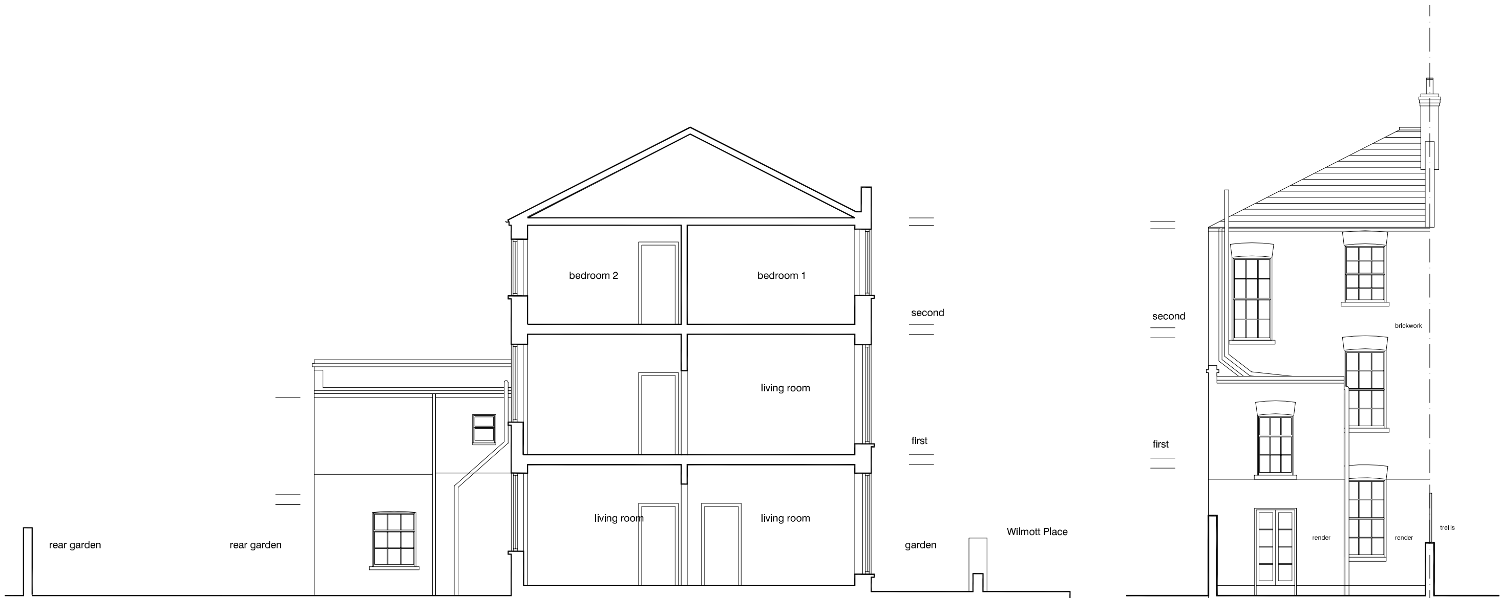
section AA as existing
