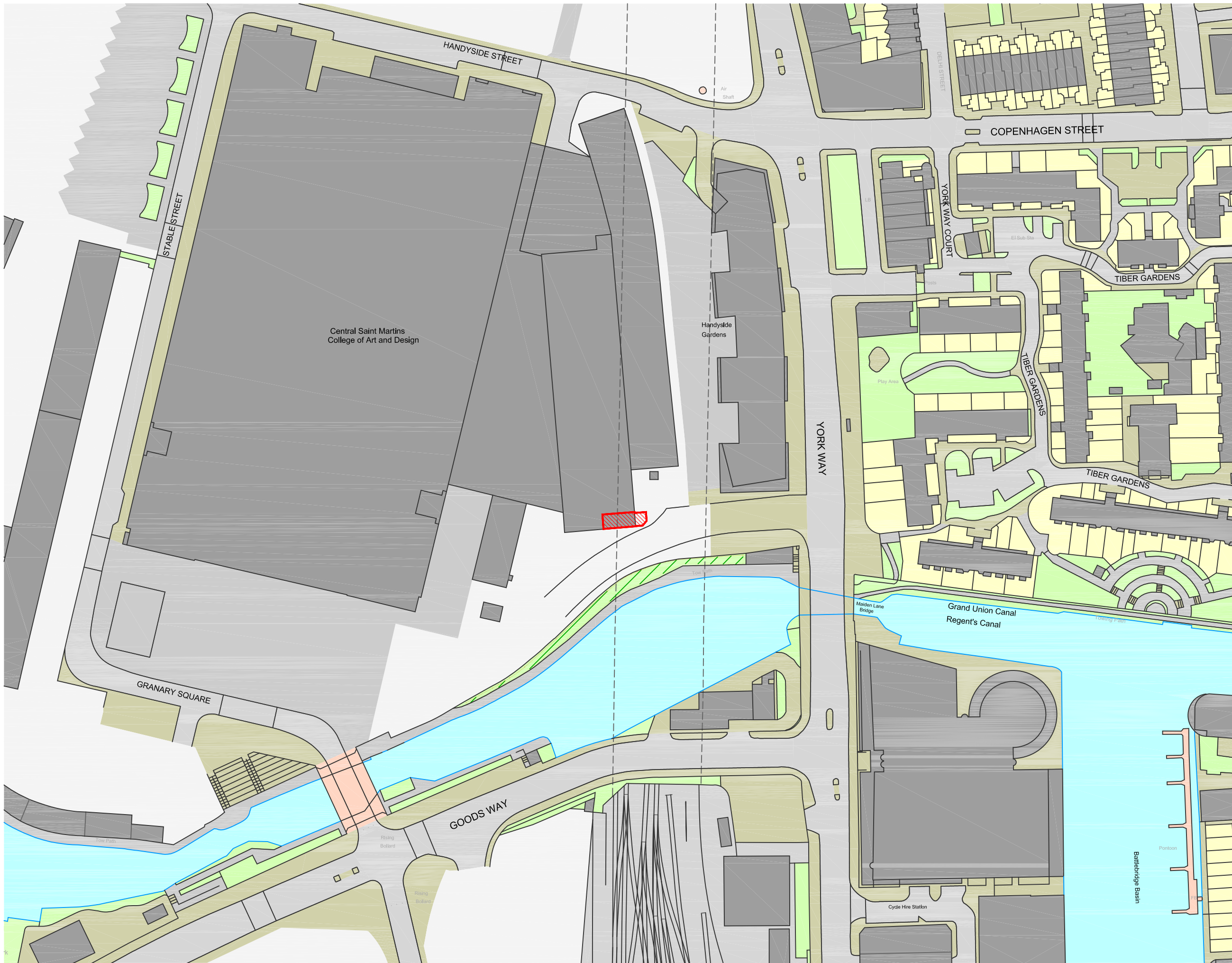
01 SITE LOCATION PLAN SCALE: 1:1250
