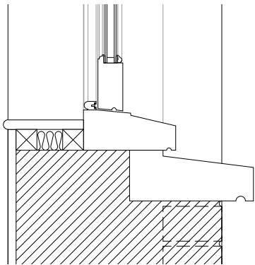
Typical Section
