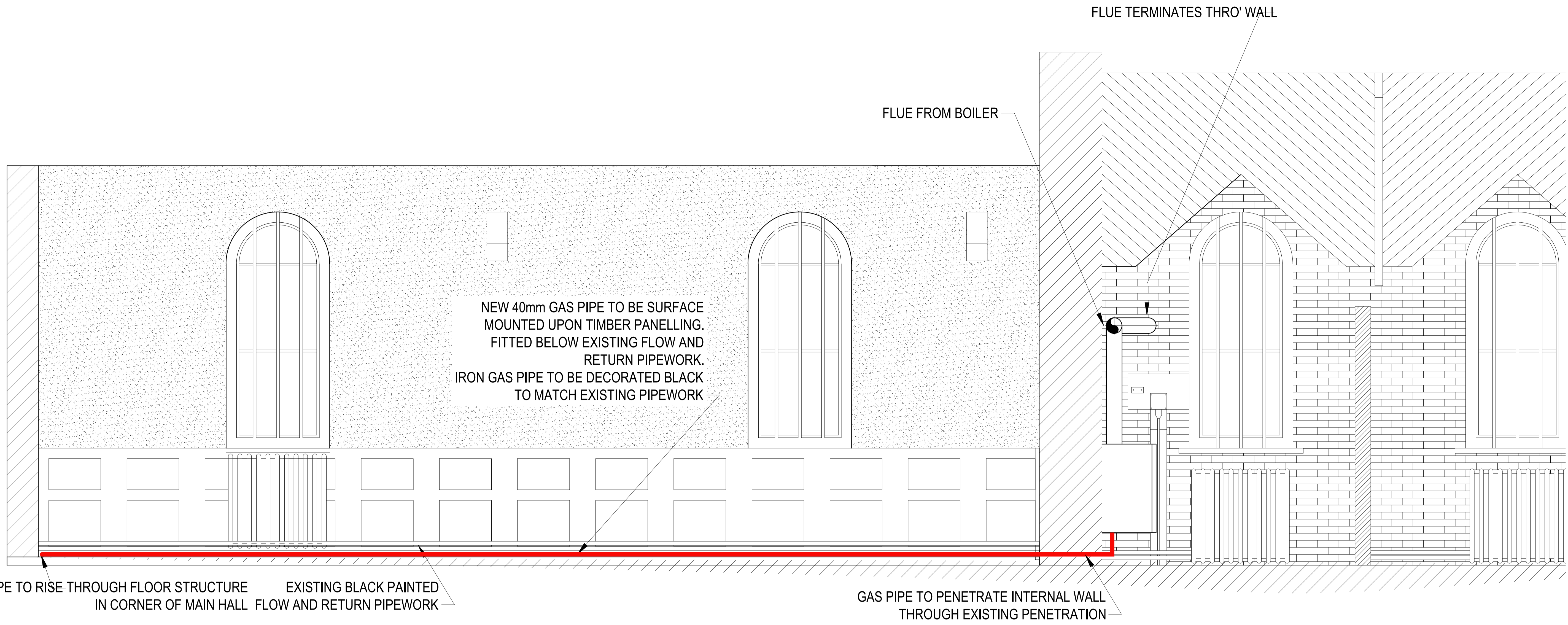
PROPOSED INTERNAL ELEVATION A SCALE @ 1:20
