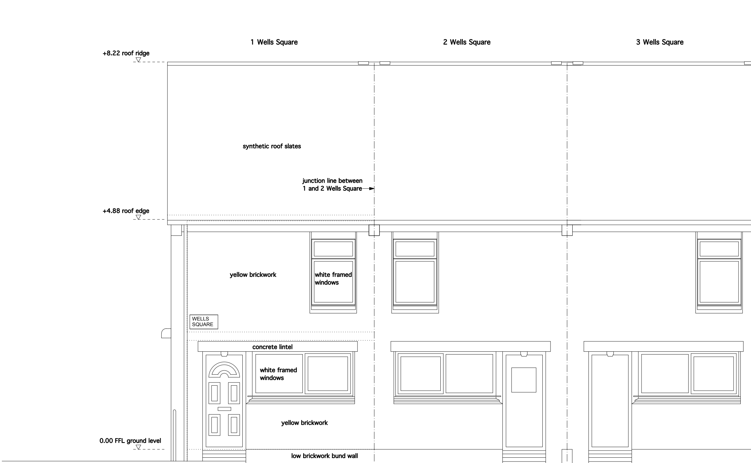
front elevation existing in context 1:50
